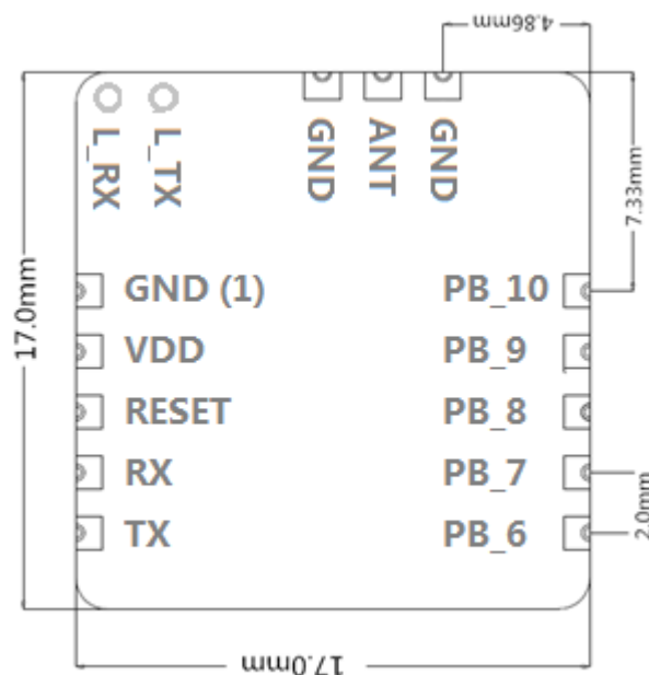
Figure 5-2 Pin configuration
