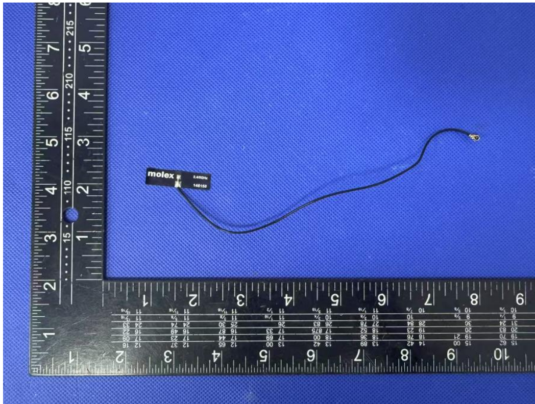
Antenna length:200mm
