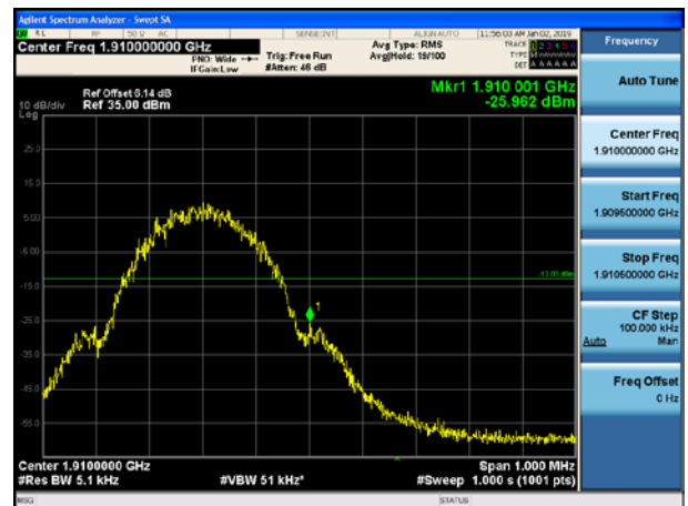
GSM 1900-HCH-GSM
