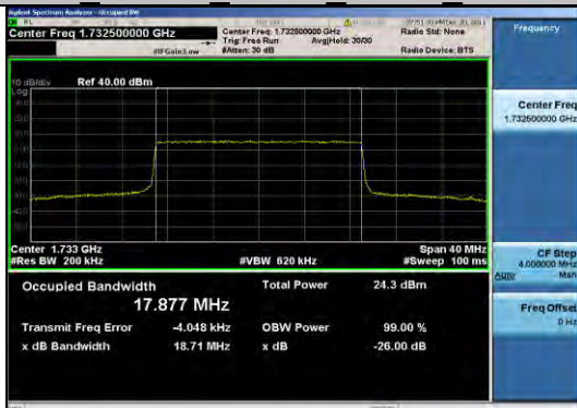
Band4_20MHz_QPSK_20175_100RB#0
