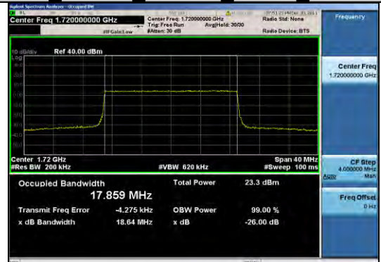
Band4_20MHz_16QAM_20175_100RB#0
