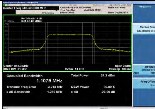
Band5 1.4MHz QPSK 20643 6RB#0
