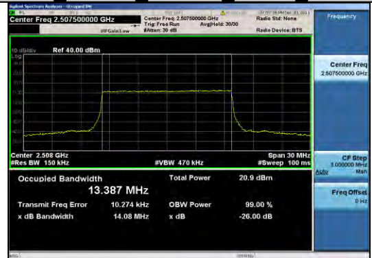
Band7 15MHz 16QAM 20825 75RB#0
