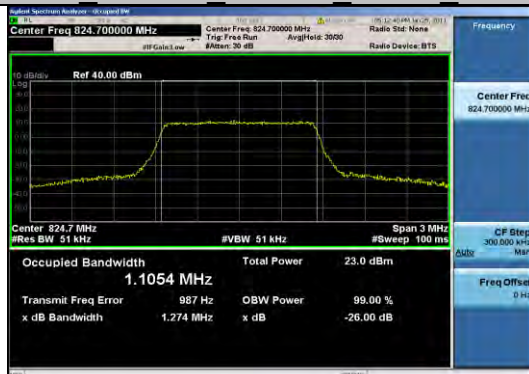
Band5 1.4MHz 16QAM 20407 6RB#0
