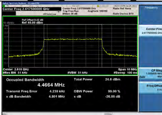
Band38 5MHz 16QAM 38225 25RB#0
