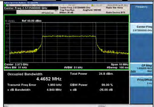
Band38 5MHz 16QAM 37775 25RB#0
