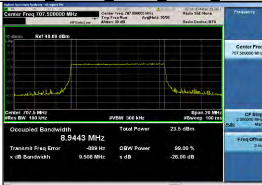
Band12_10MHz_QPSK_23095_50RB#0
