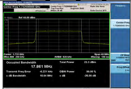
Band4_20MHz_16QAM_20300_100RB#0
