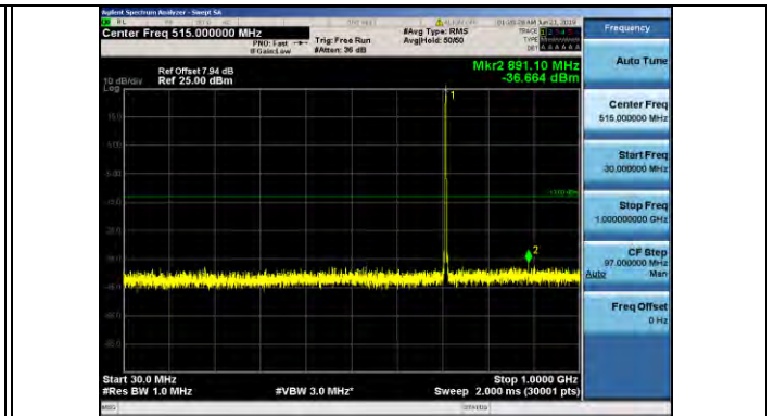
Band12 1.4MHz 16QAM 23173 1RB#0
