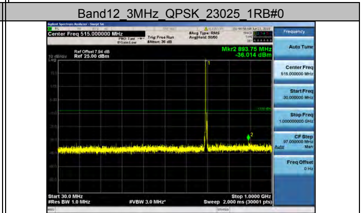
Band12 3MHz QPSK 23025 1RB#0
