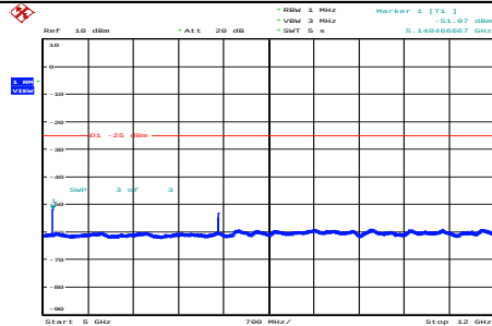
Band38-5MHz-QPSK-37775-1RB#0-Range5:5000~12000MHz
