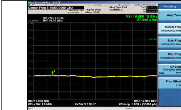
Band17 5MHz 16QAM 23790 1RB#0
