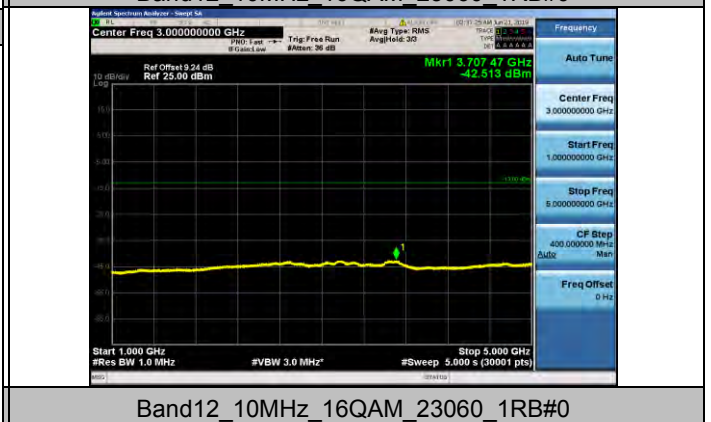
Band12 10MHz 16QAM 23060 1RB#0
