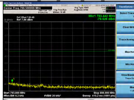
Band13 5MHz 16QAM 23255 1RB#0
