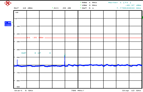
Band38-5MHz-QPSK-38000-1RB#0-Range5:5000~12000MHz
