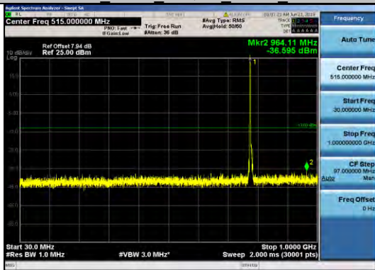
Band13 5MHz 16QAM 23230 1RB#0
