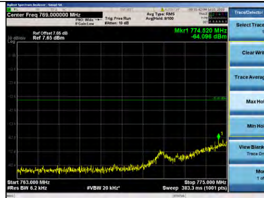
Band13 5MHz 16QAM 23230 1RB#0
