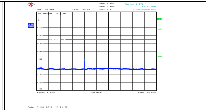
Band41_20MHz_16QAM_40740_1RB#0
