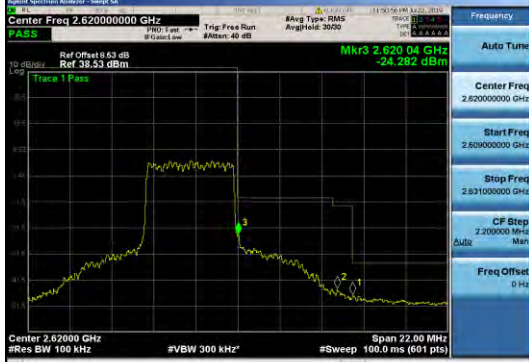
Band38 5MHz QPSK 38225 25RB#0
