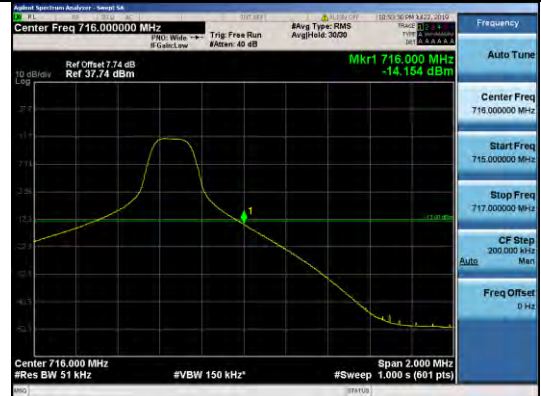
Band12 5MHz 16QAM 23155 25RB#0
