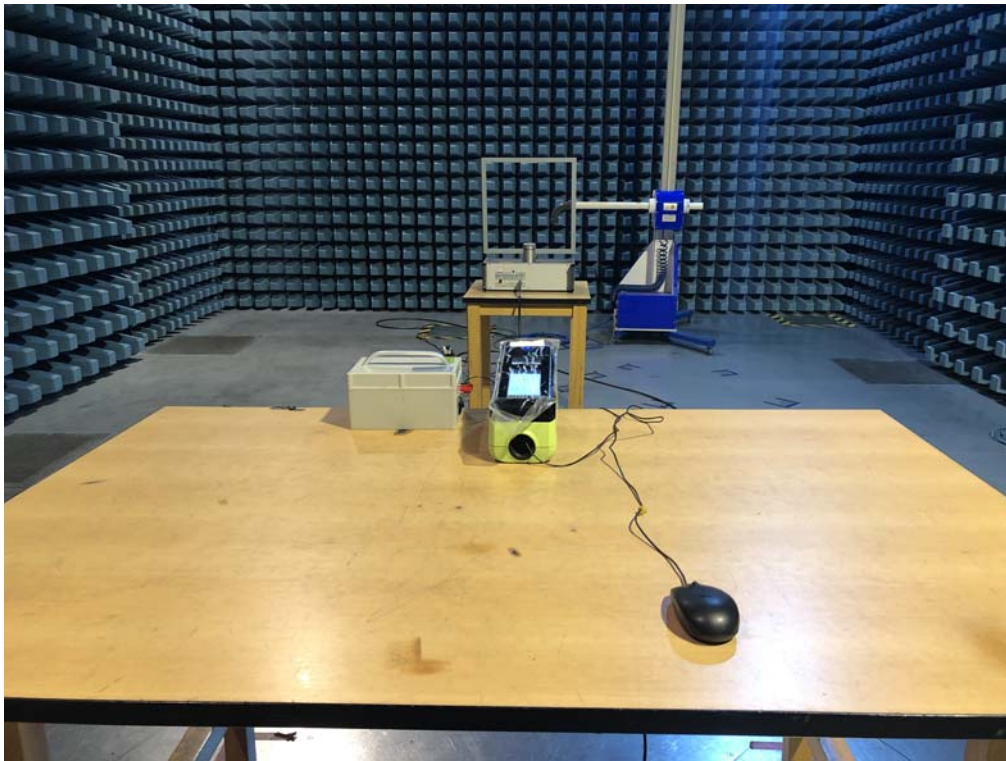
FCC Part15C Radiated Emission below 30MHz -Front
