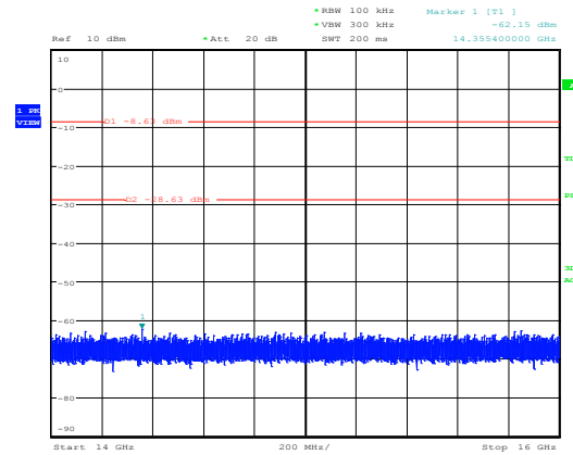
Conducted spurious emissions, mode 3-DH5, C2 Date: 15.JAN.2016 11:08:06
