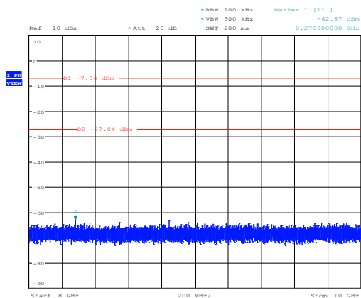
Conducted spurious emissions, mode 3-DH5, A2 Date: 15.JAN.2016 10:49:39
