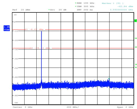
Conducted spurious emissions, mode 3-DH5, C2 Date: 15.JAN.2016 11:05:33
