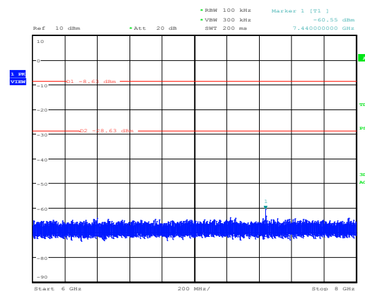
Conducted spurious emissions, mode 3-DH5, C2 Date: 15.JAN.2016 11:05:33
