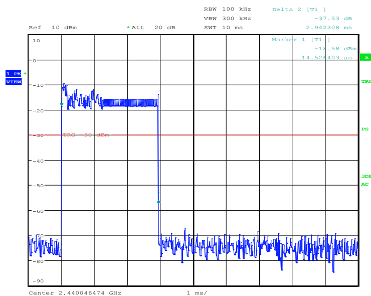
Figure 28: Dwell Time, Mode D (Hopping), DH5, EDR (8DPSK)
