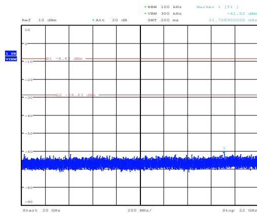
Conducted spurious emissions, mode 3-DH5, C2 Date: 15.JAN.2016 11:08:26
