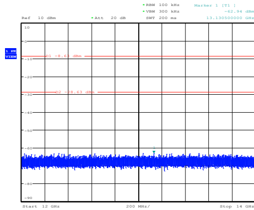
Conducted spurious emissions, mode 3-DH5, C2 Date: 15.JAN.2016 11:07:32
