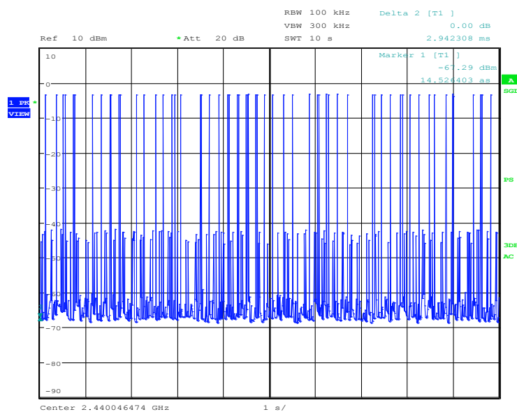
Figure 24: Number of Hops, Mode D (Hopping), DH3, BDR (GFSK)
