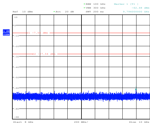
Conducted spurious emissions, mode 3-DH5, B2 Date: 15.JAN.2016 10:58:31
