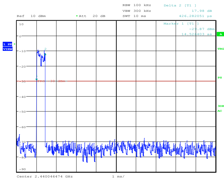
Figure 26: Dwell Time, Mode D (Hopping), DH1, EDR (8DPSK)
