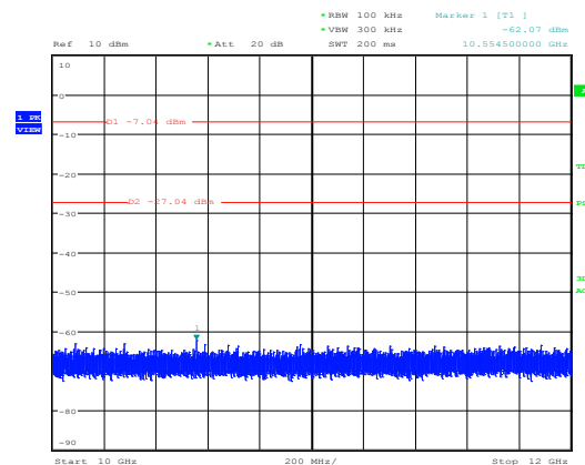
Conducted spurious emissions, mode 3-DH5, A2 Date: 15.JAN.2016 10:49:58
