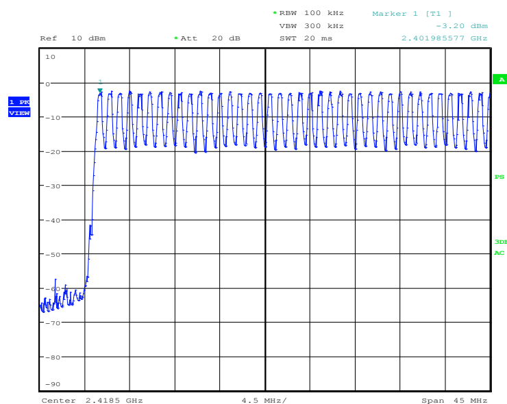
Figure 16: Hopping Frequencies up to 2440MHz, Mode D (Hopping), BDR (GFSK)
