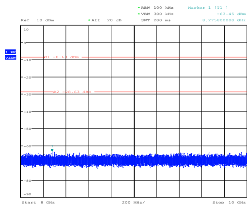
Conducted spurious emissions, mode 3-DH5, C2 Date: 15.JAN.2016 11:05:51
