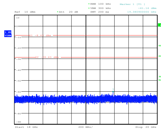
Conducted spurious emissions, mode 3-DH5, C2 Date: 15.JAN.2016 11:08:06
