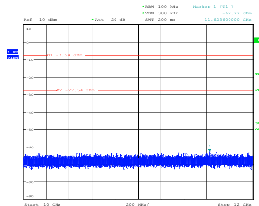
Conducted spurious emissions, mode 3-DH5, B2 Date: 15.JAN.2016 10:58:50
