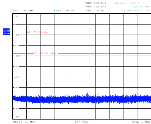
Conducted spurious emissions, mode 3-DH5, B2 Date: 15.JAN.2016 10:56:54
