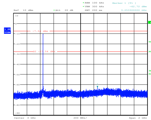
Conducted spurious emissions, mode 3-DH5, B2 Date: 15.JAN.2016 10:58:13
