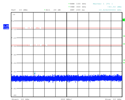
Conducted spurious emissions, mode 3-DH5, C2 Date: 15.JAN.2016 11:06:32
