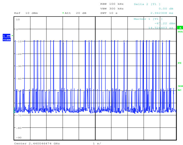
Figure 30: Number of Hops, Mode D (Hopping), DH3, EDR (8DPSK)
