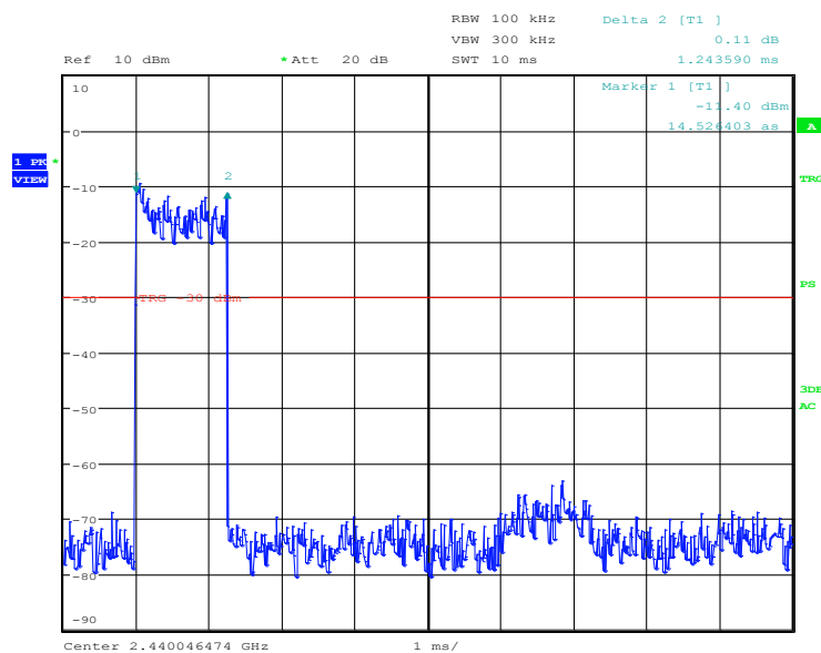
Figure 27: Dwell Time, Mode D (Hopping), DH3, EDR (8DPSK)
