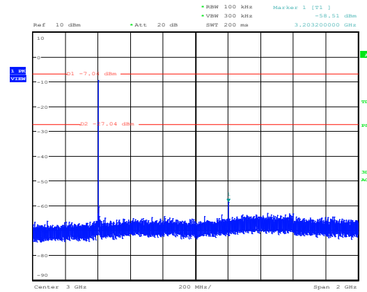
Conducted spurious emissions, mode 3-DH5, A2 Date: 15.JAN.2016 10:49:13
