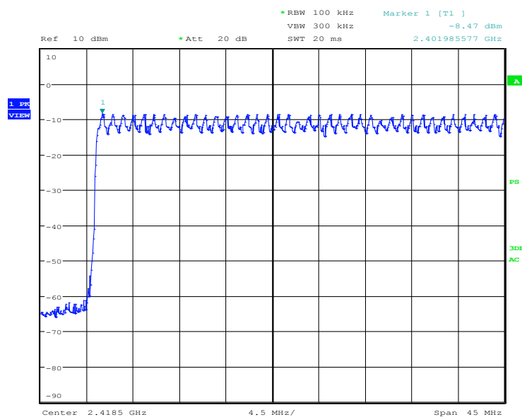
Figure 18: Hopping Frequencies up to 2440MHz, Mode D (Hopping), EDR (8DPSK)
