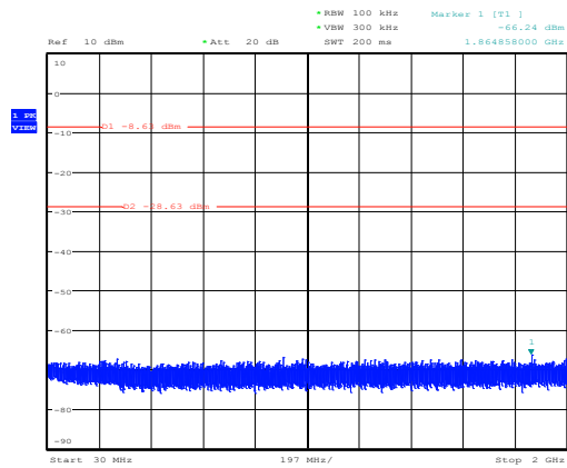
Conducted spurious emissions, mode 3-DH5, C2 Date: 15.JAN.2016 11:04:51
