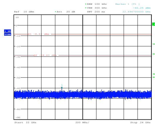
Conducted spurious emissions, mode 3-DH5, C2 Date: 15.JAN.2016 11:08:43
