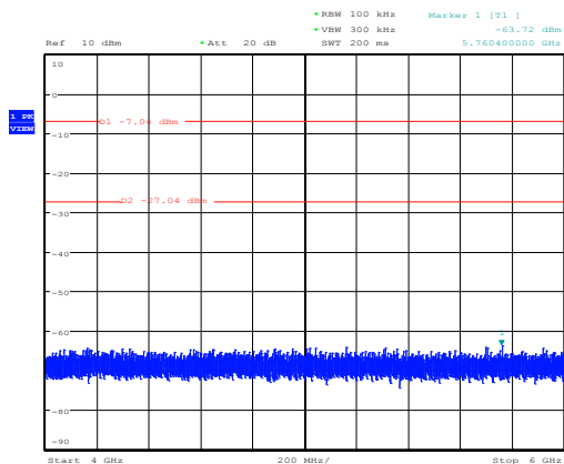
Conducted spurious emissions, mode 3-DH5, A2 Date: 15.JAN.2016 10:48:42
