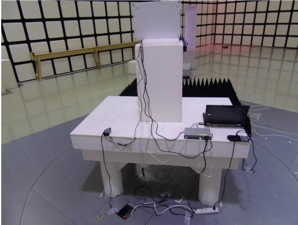
Photograph 7: Set-up for Radiated Emission of Transmitter above 1GHz, Front View
