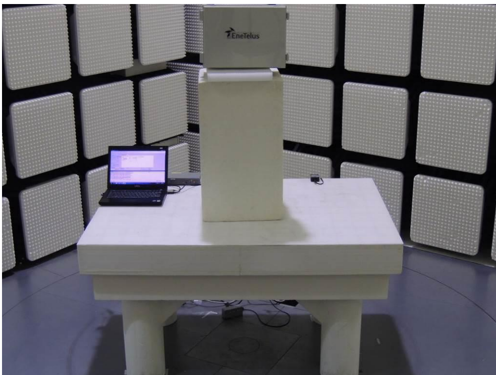
Photograph 6: Set-up for Radiated Emission of Transmitter above 1GHz, Front View
