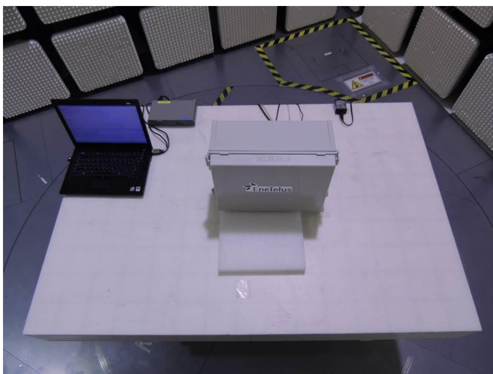
Photograph 4: Set-up for Radiated Emission of Transmitter below 1GHz band, Front View
