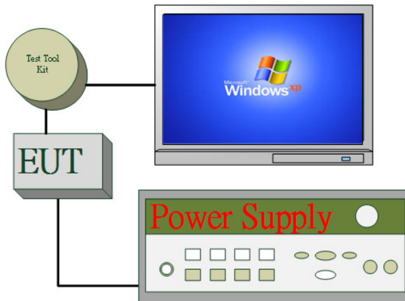
Fig. 2-1 Radiated Emission & Conducted (Antenna Port) Configuration
