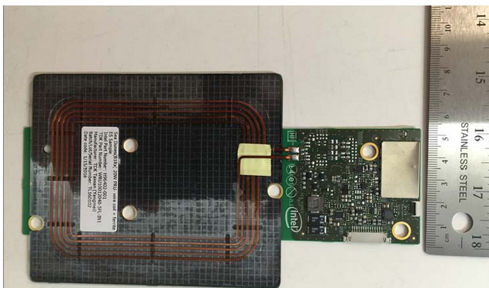
Top view of board with shield over Bluetooth circuitry
