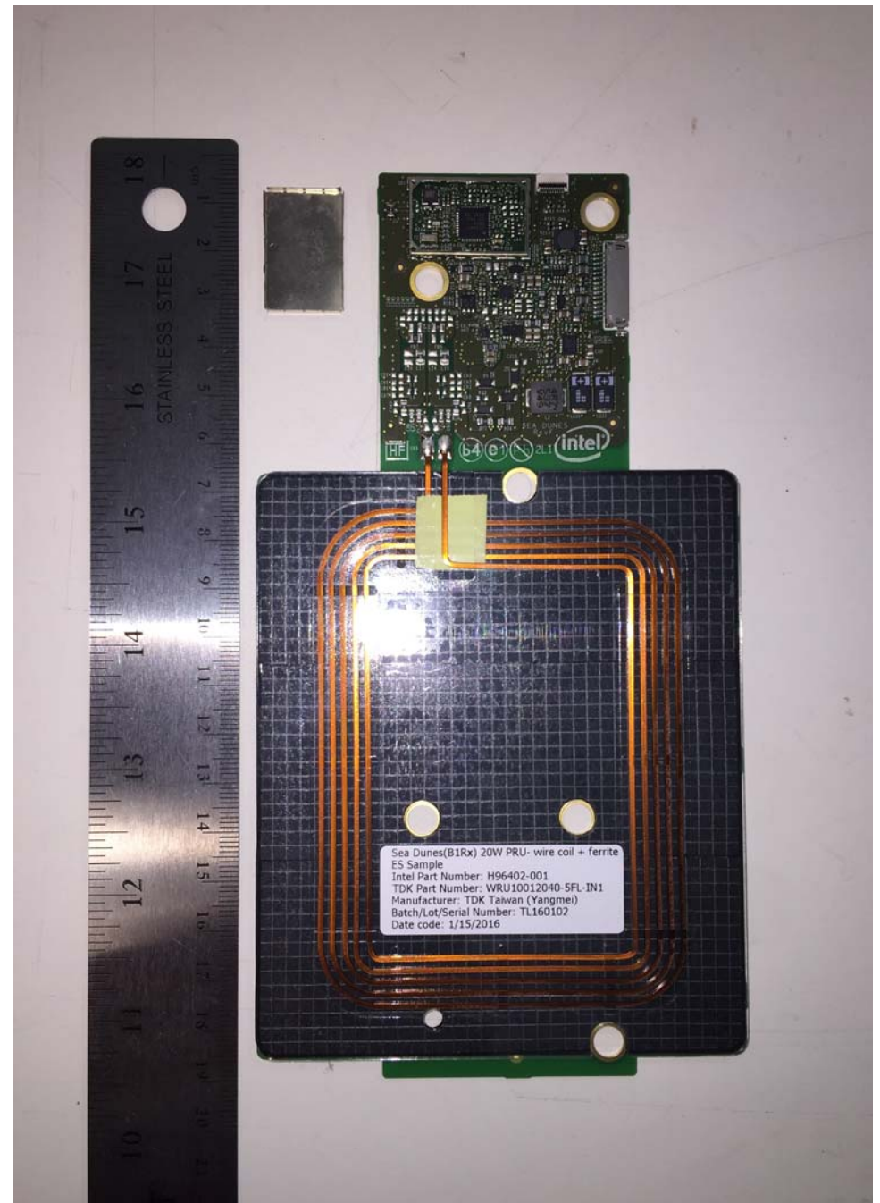
Top View of Board with shield over Bluetooth circuitry removed
