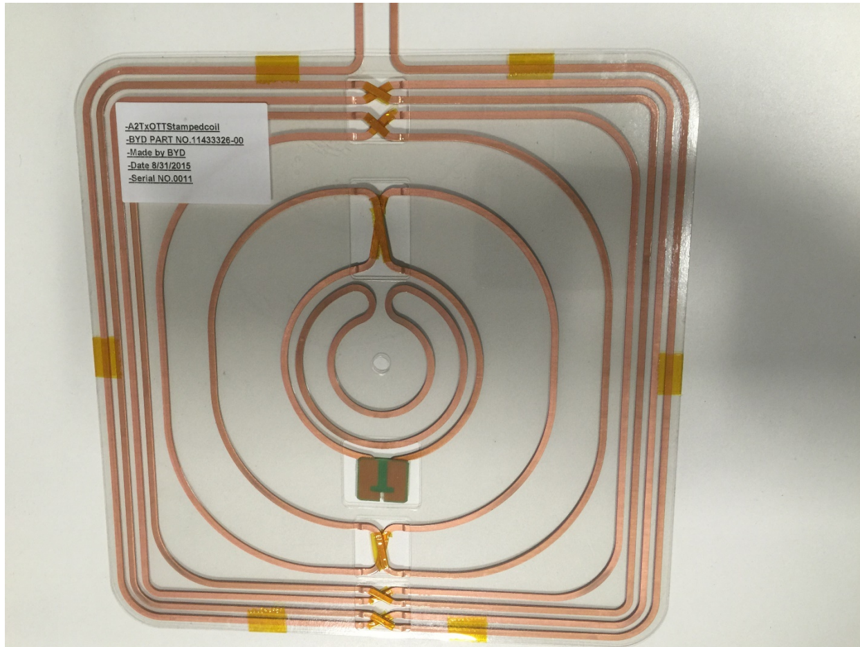
Top View of Coil
