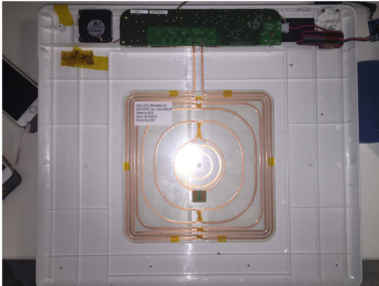
Internal Construction View with top removed
