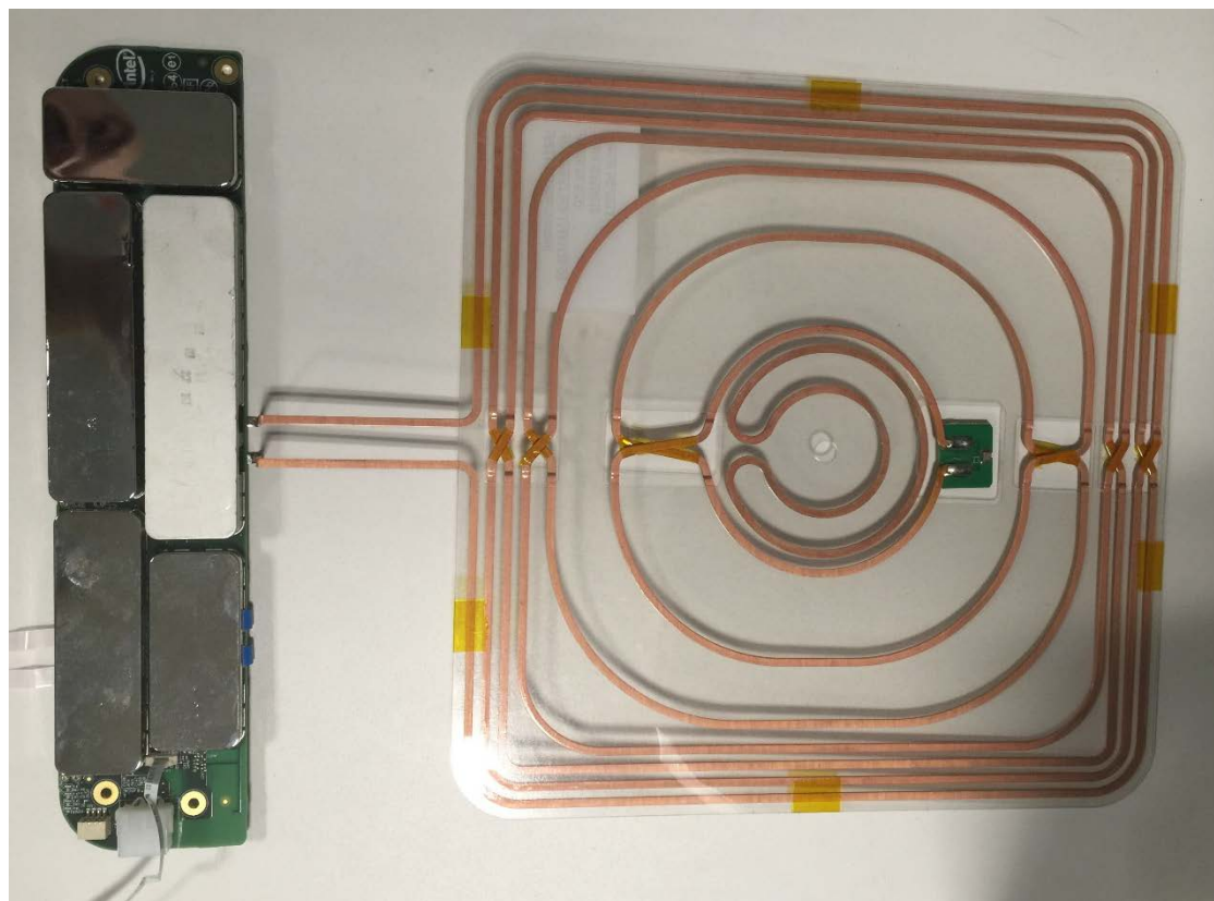
Main Circuit Board – Top View with Shields; Bottom View of Coil
