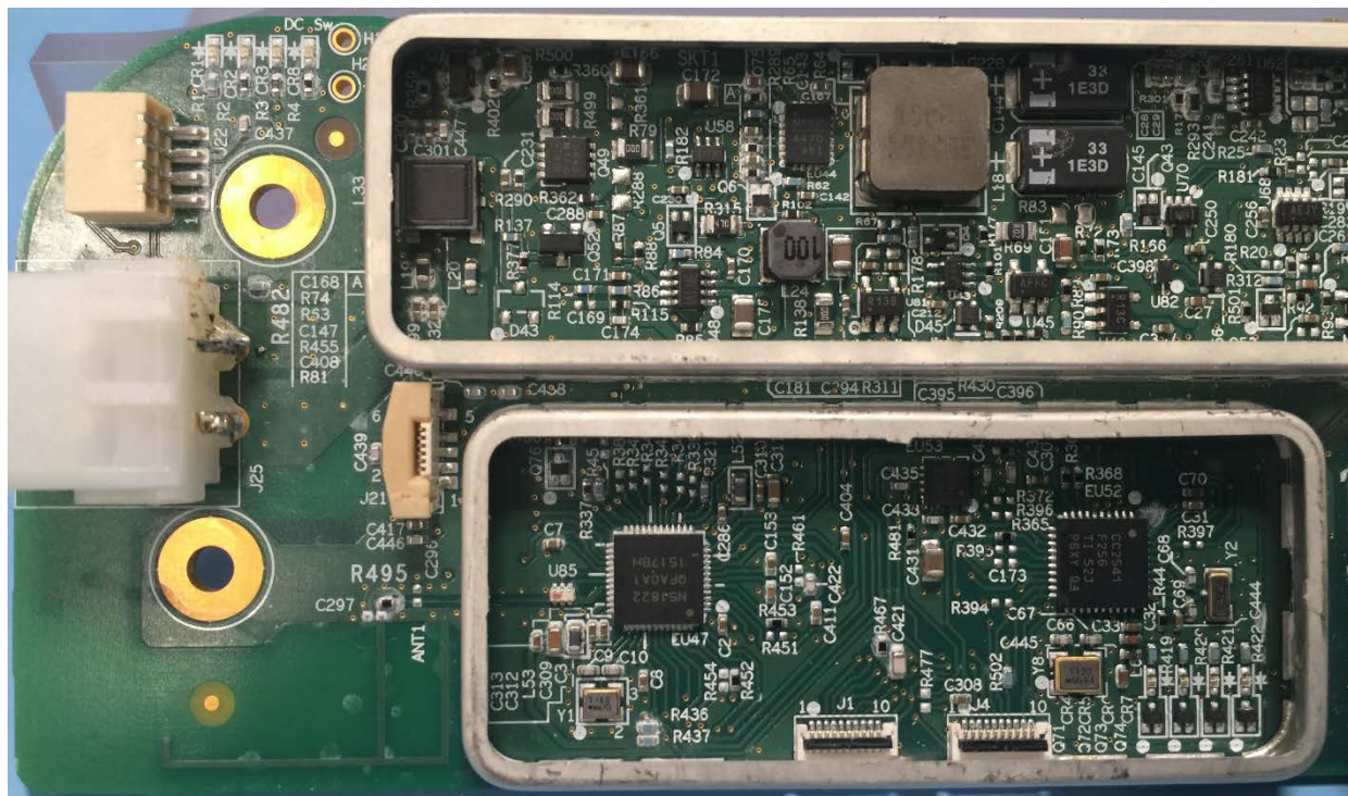
Main Circuit Board – Top View, Shields Removed – Bluetooth Trace Antenna (ANT1) and Bluetooth Circuitry (bottom); DC-DC Power Supply Circuitry (Top)
