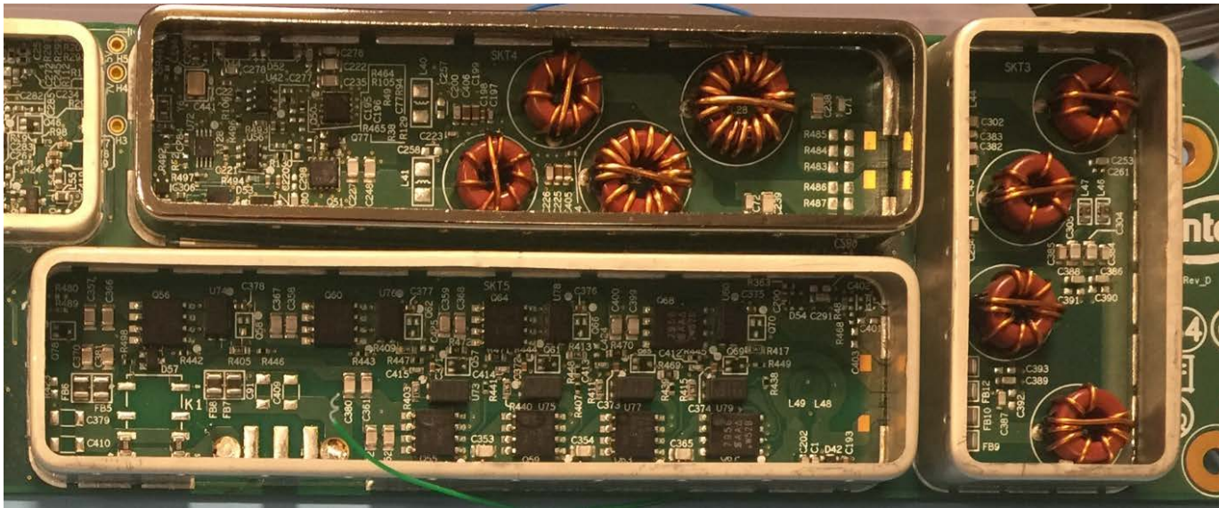
Main Circuit Board – Top View, Shields Removed (Close up – 6.78MHz Circuitry)
