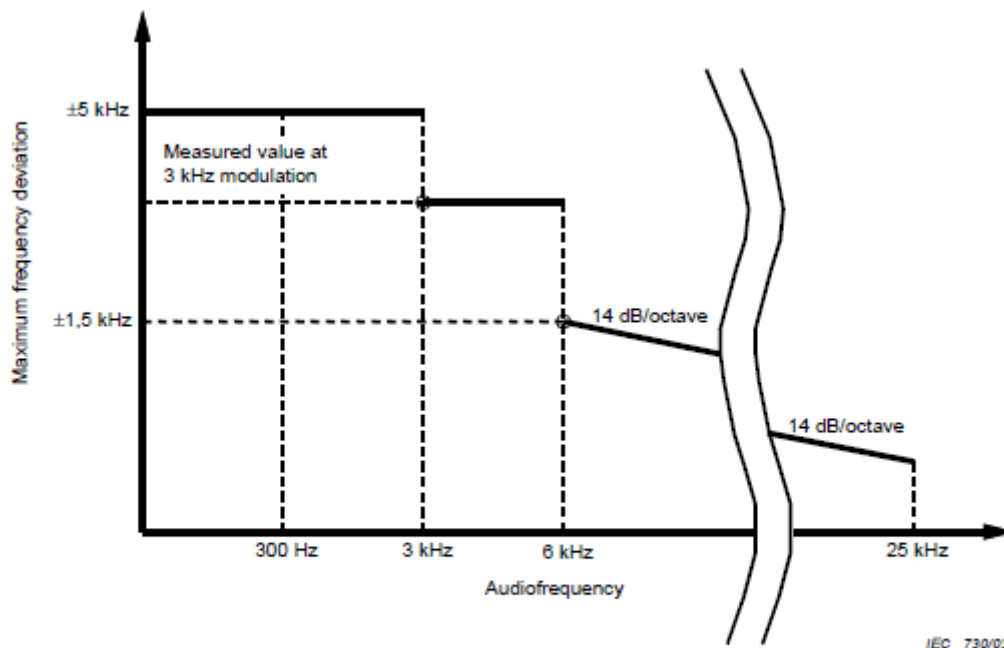
Figure 1 – Frequency deviation
