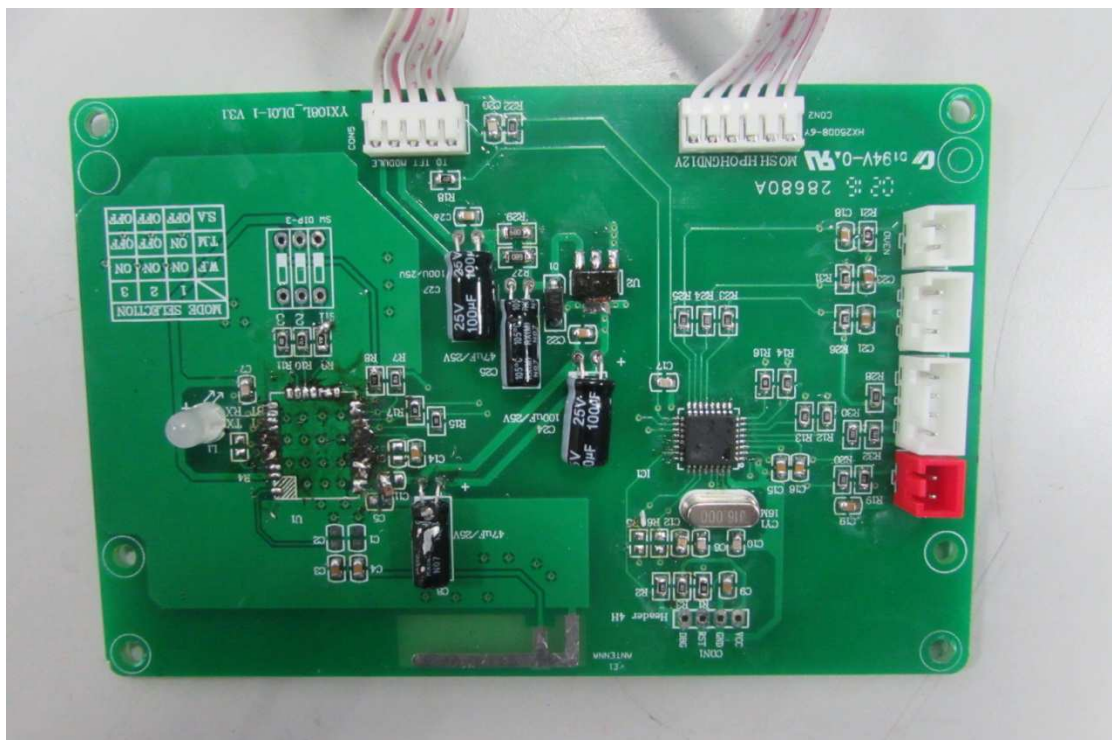
The control circuit PCB view (Remove Bluetooth module)
