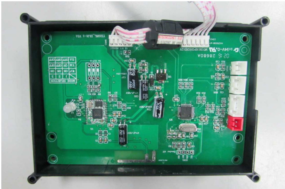
The control circuit box view
