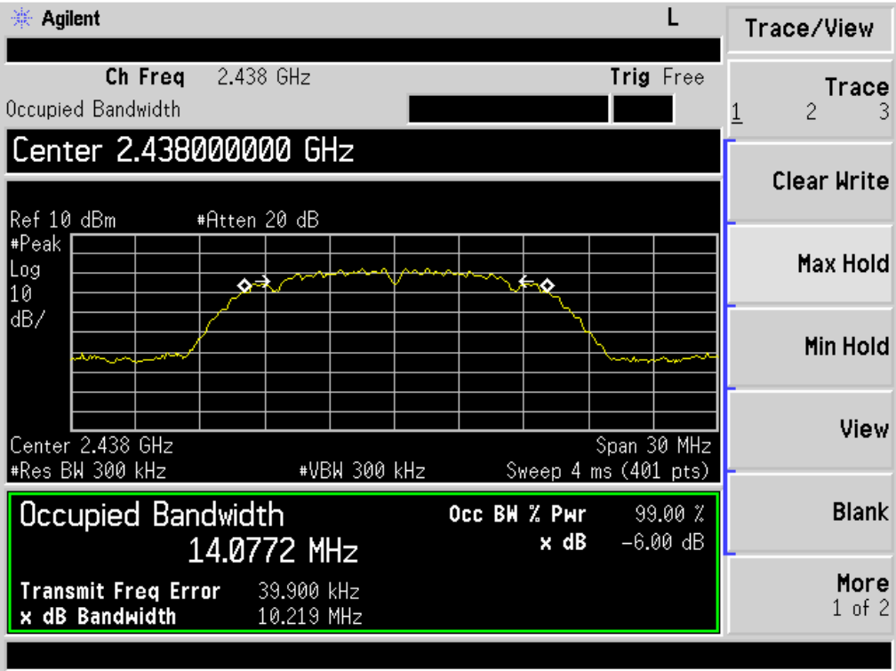
Middle channel 2438MHz
