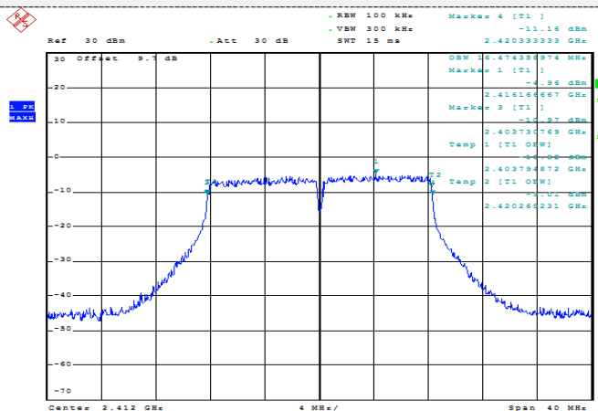
802.11g
