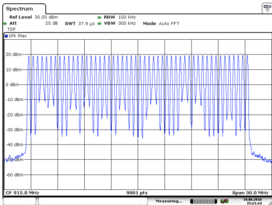
Figure 25. 50 channels
