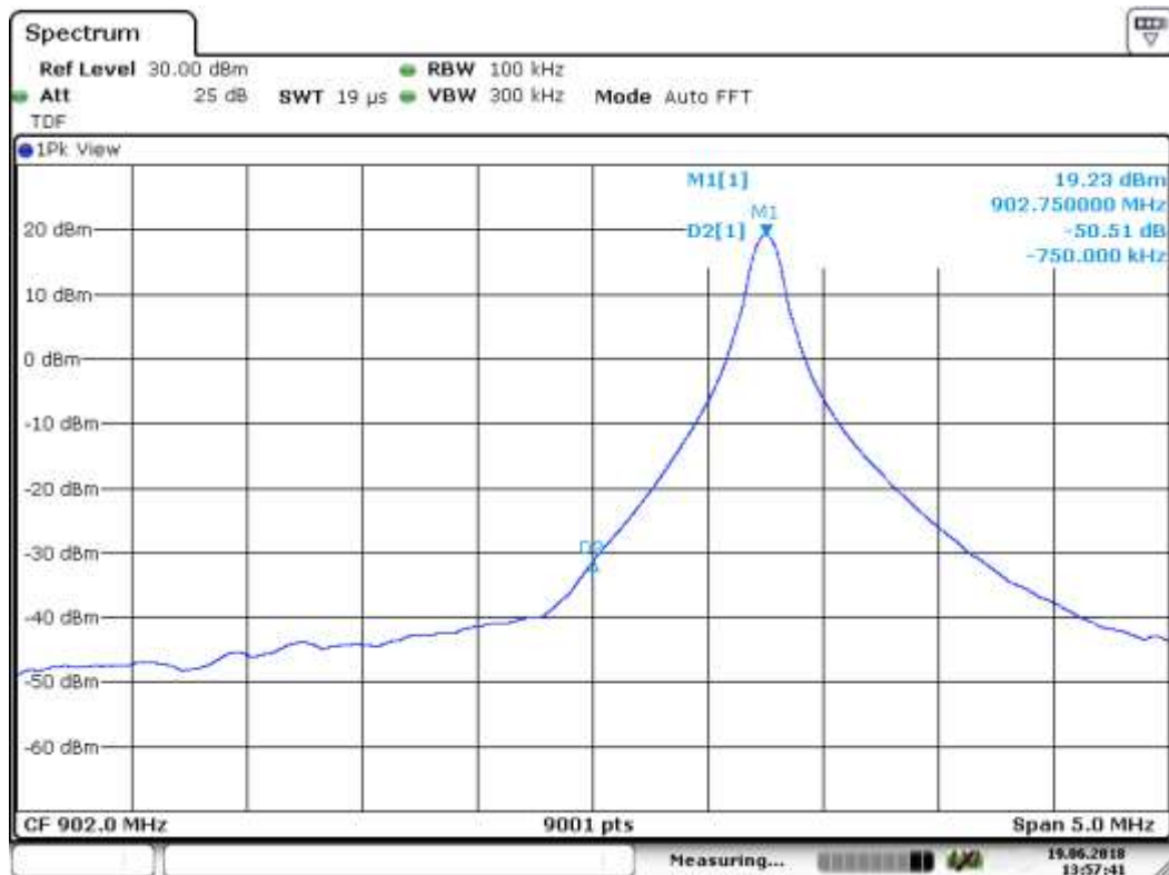
Figure 17. Conducted emission at low band edge hopping disabled
