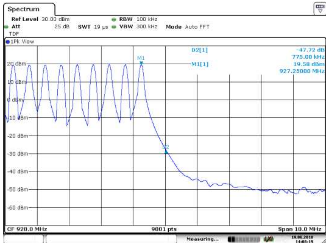
Figure 20. Conducted emission at high band edge hopping enabled
