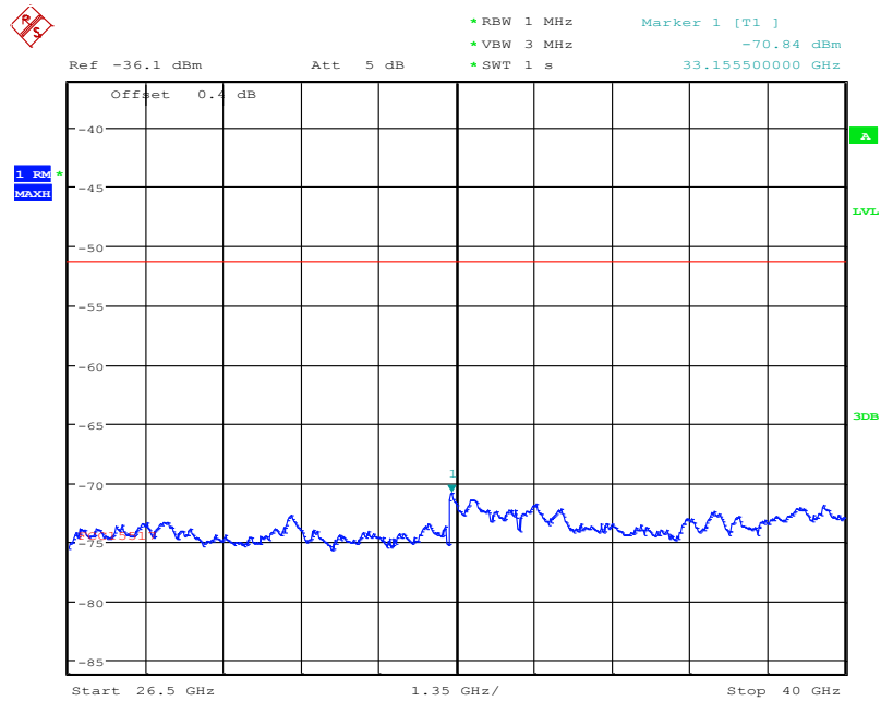
Plot 95: TX radiated, 26.5 GHz to 40 GHz, channel 1 (bottom)
