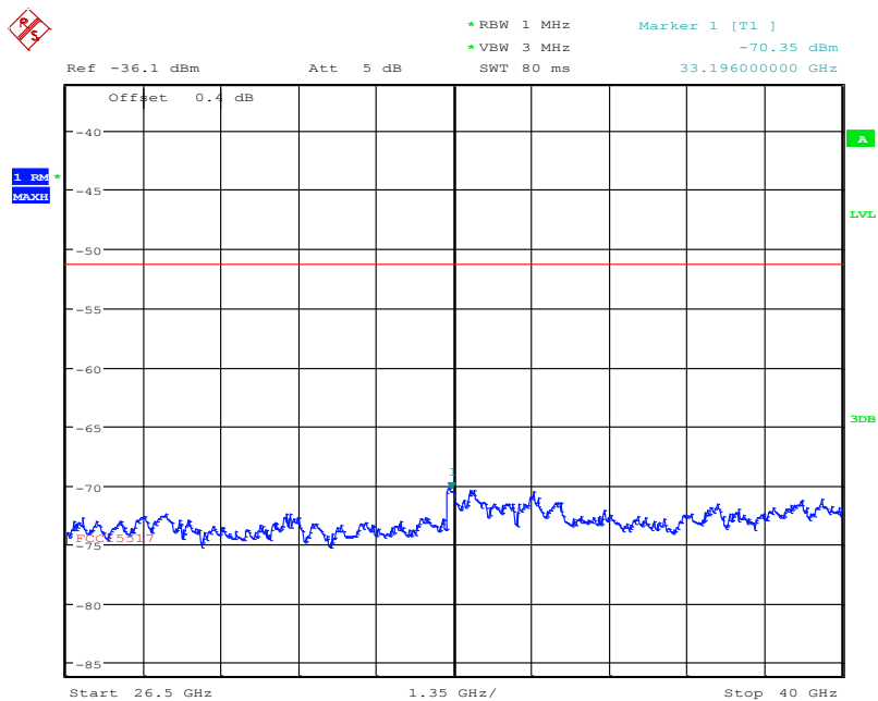
Plot 97: TX radiated, 26.5 GHz to 40 GHz, channel 6 (top)
