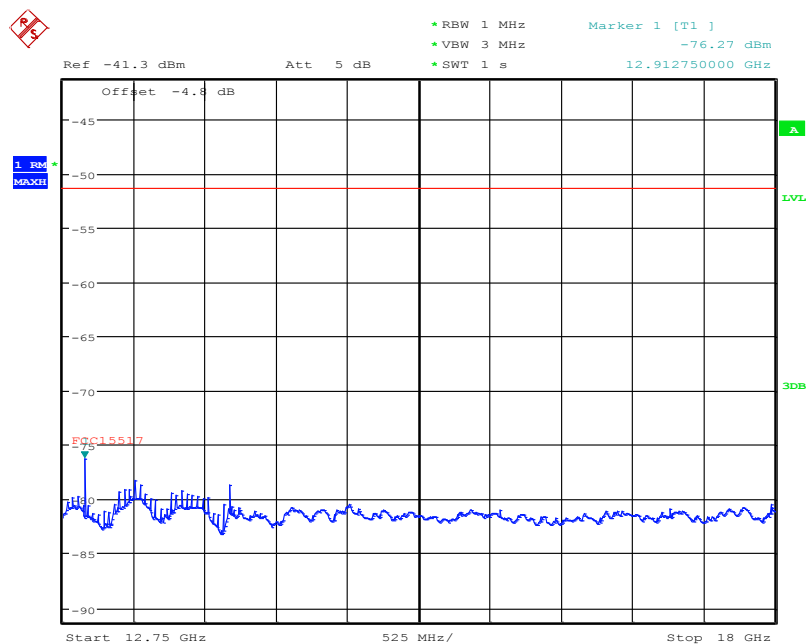
Plot 89: TX radiated, 12.75 GHz to 18 GHz, channel 1 (bottom)
