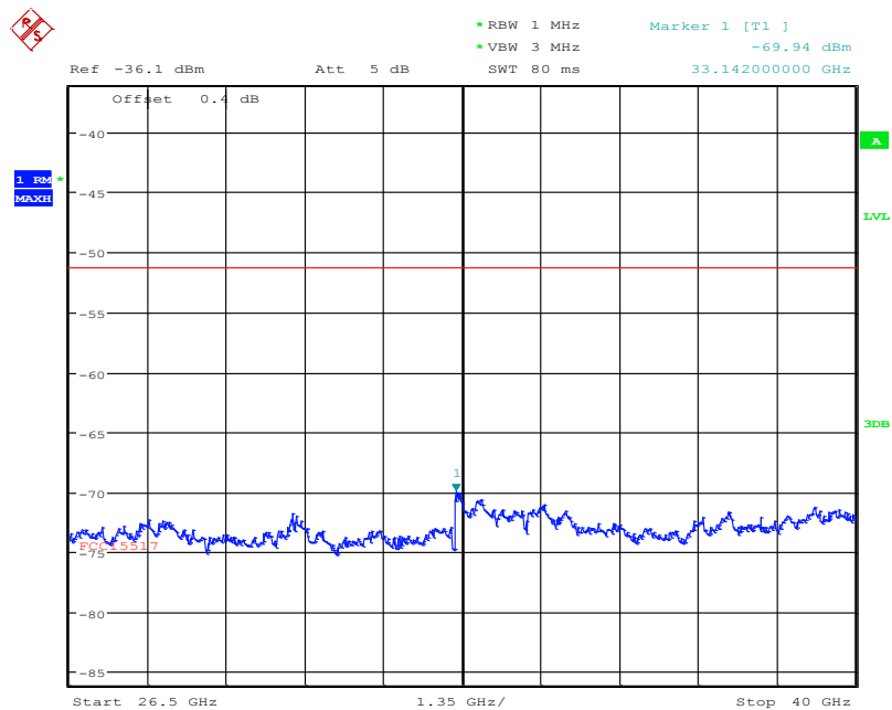
Plot 96: TX radiated, 26.5 GHz to 40 GHz, channel 3 (middle)
