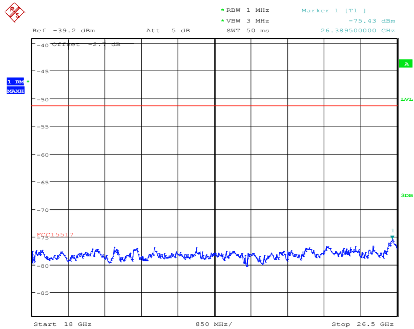
Plot 93: TX radiated, 18 GHz to 26.5 GHz, channel 3 (middle)
