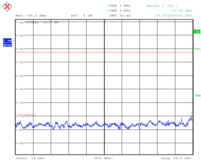
Plot 94: TX radiated, 18 GHz to 26.5 GHz, channel 6 (top)
