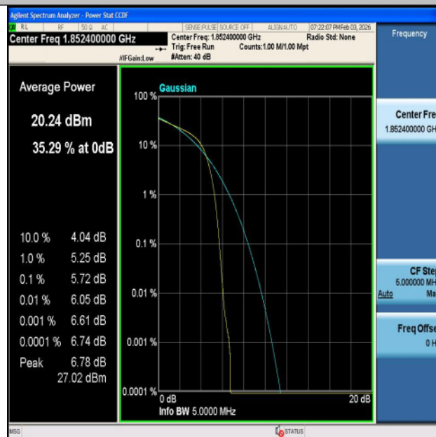
Band2-9262-3-PASS
