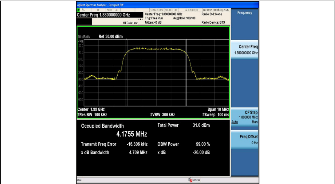
Band2-9400-2-PASS
