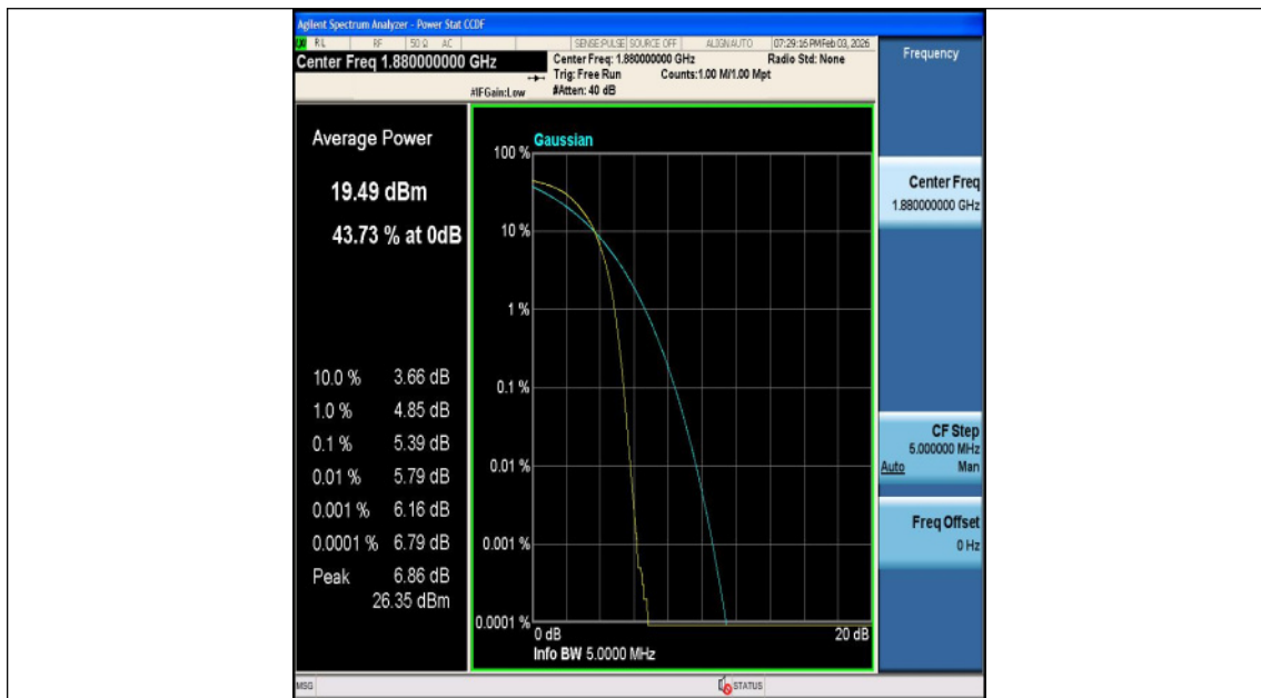
Band2-9400-5-PASS
