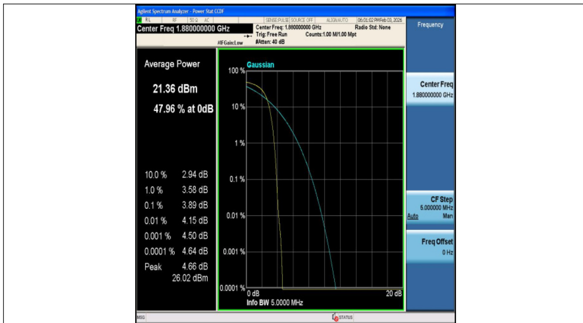
Band2-9400-4-PASS
