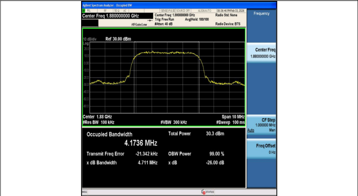
Band2-9400-3-PASS
