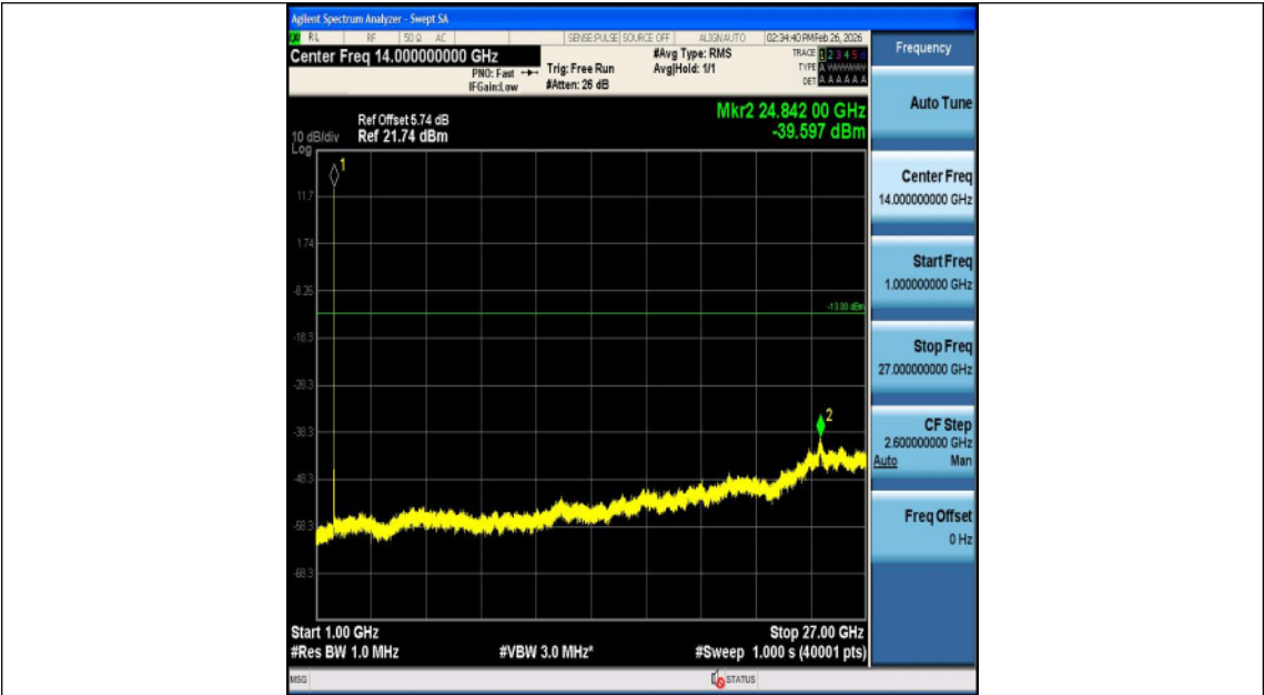
Band2-9262-2-3000~20000MHz-PASS
