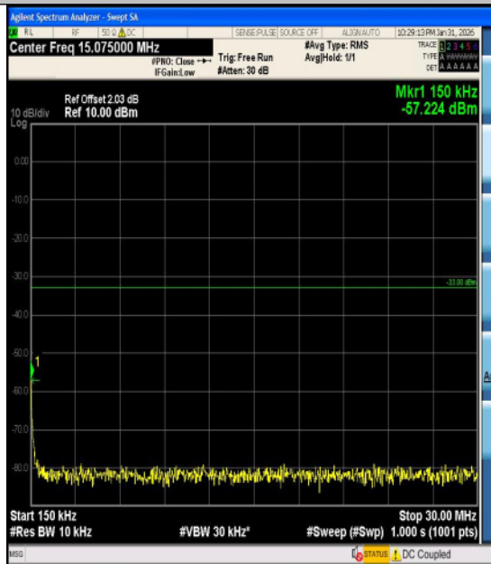
Band2-10MHz-QPSK-18900-1RB#0-1000~3000- PASS
