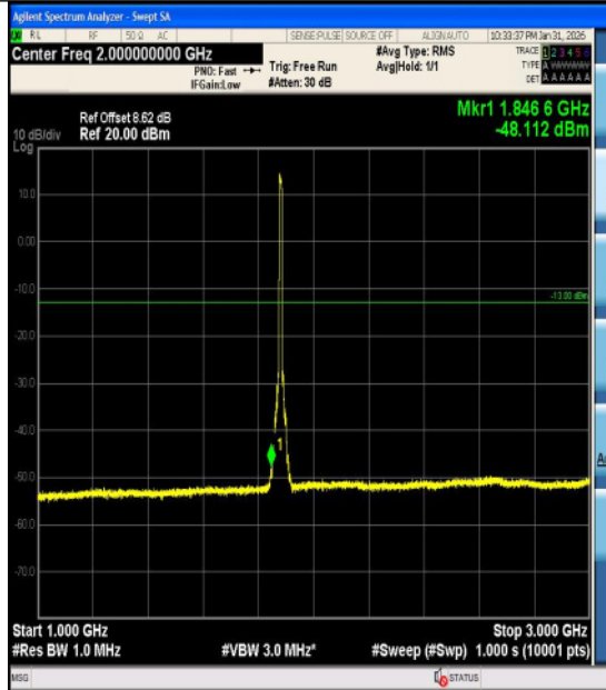
Band2-10MHz-16QAM-18900-1RB#0-0.009~0.1 5-PASS
