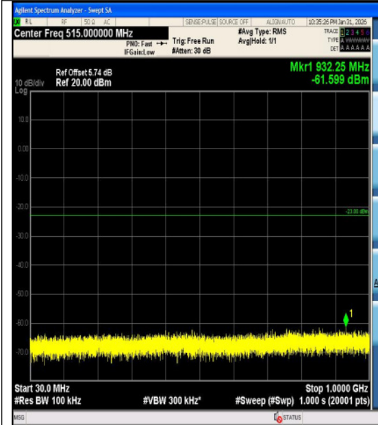
Band2-10MHz-QPSK-19150-1RB#0-3000~2000 0-PASS
