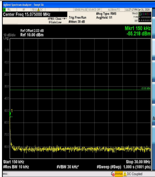
Band2-15MHz-QPSK-19125-75RB#0-1000~300 0-PASS
