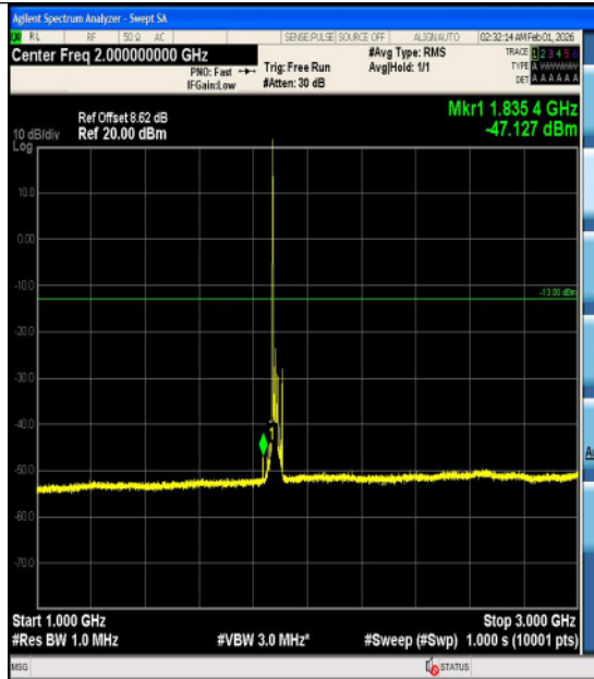
Band2-20MHz-QPSK-18900-1RB#99-0.009~0.1 5-PASS
