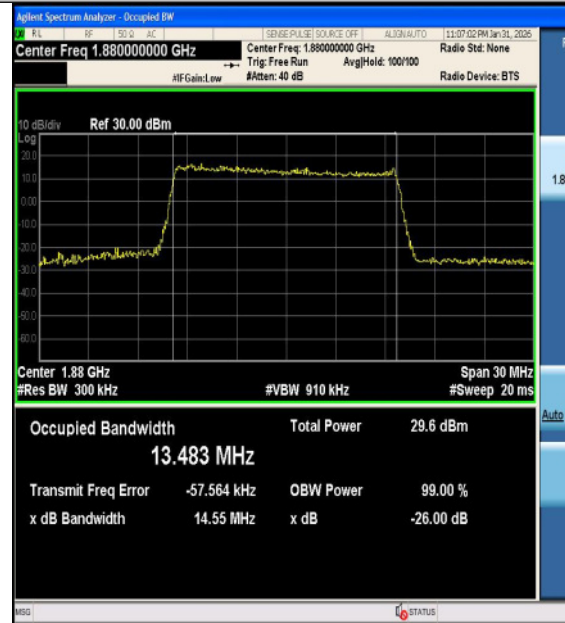
Band2-15MHz-16QAM-19125-75RB#0-PASS
