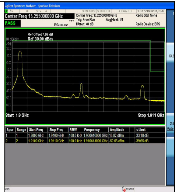
Band2-10MHz-16QAM-19150-50RB#0-PASS
