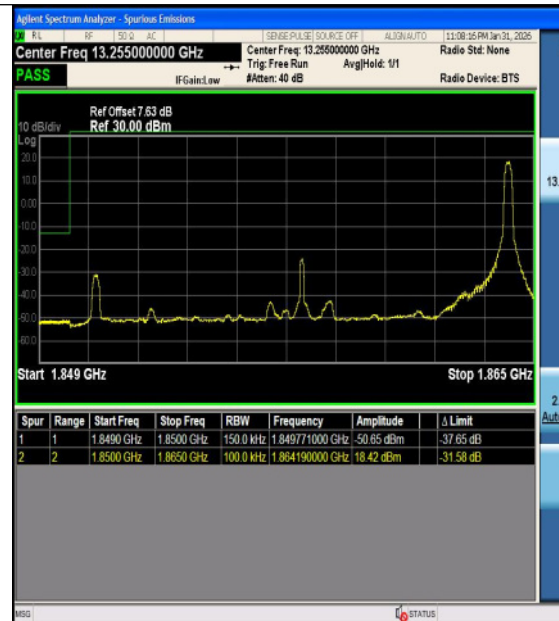
Band2-15MHz-16QAM-18675-1RB#0-PASS
