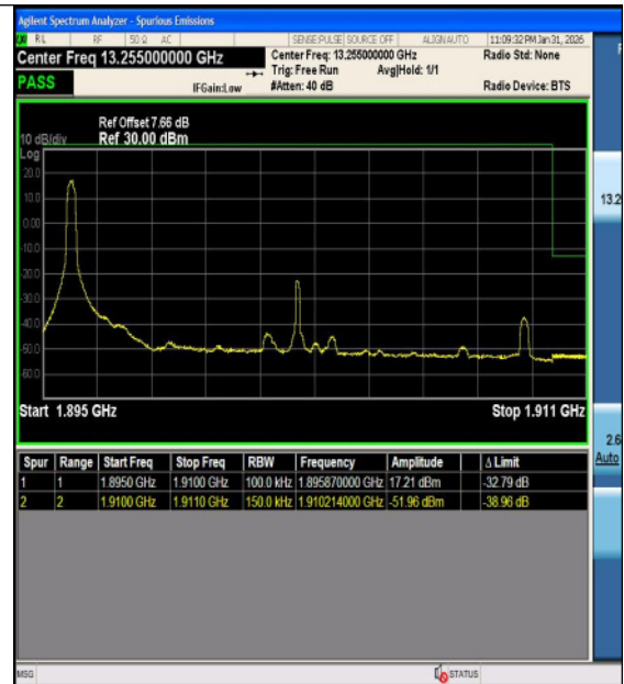
Band2-15MHz-16QAM-19125-75RB#0-PASS
