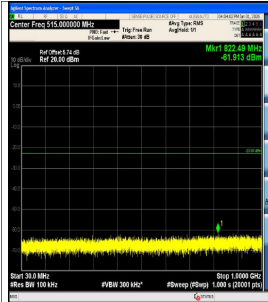
Band2-1.4MHz-QPSK-18607-1RB#0-3000~2000 0-PASS
