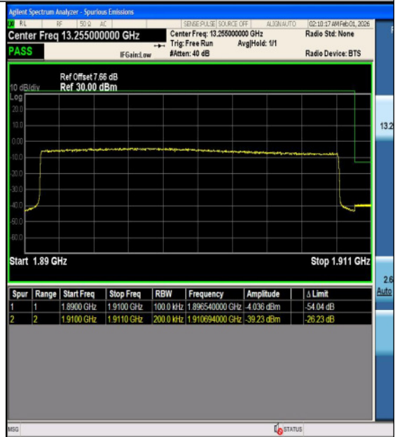
Band2-20MHz-16QAM-19100-100RB#0-PASS
