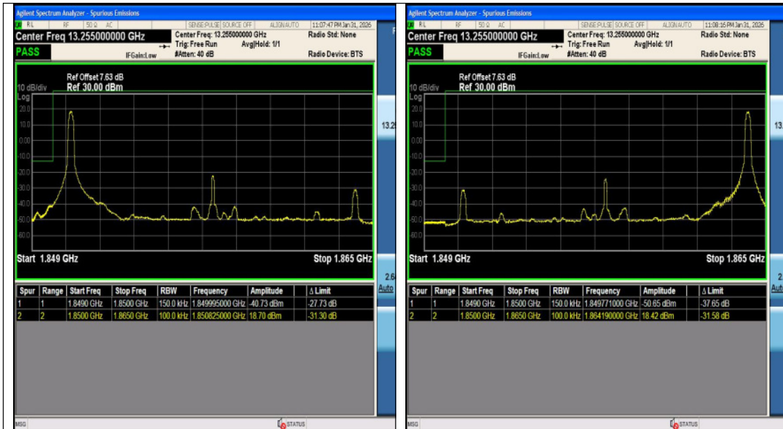
Band2-15MHz-QPSK-18675-75RB#0-PASS
