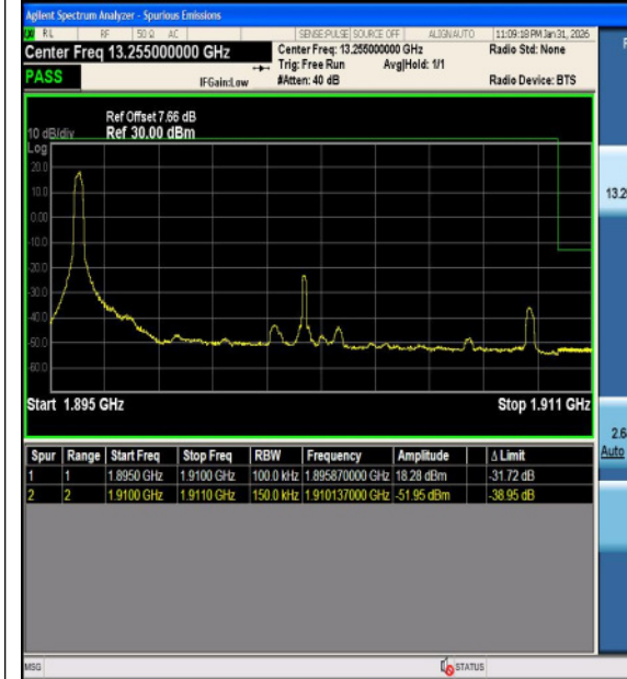
Band2-15MHz-QPSK-19125-75RB#0-PASS
