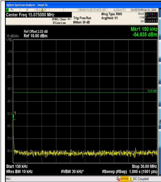
Band2-1.4MHz-QPSK-18607-1RB#5-1000~3000 -PASS
