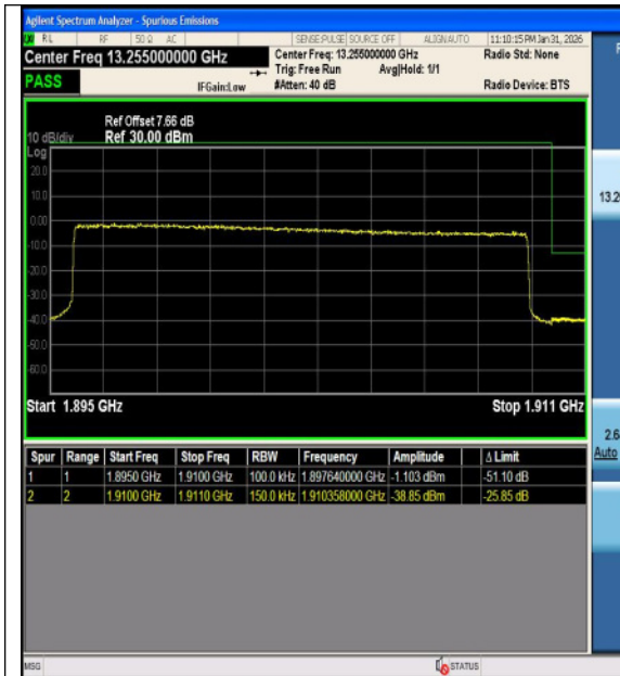
Band2-15MHz-16QAM-19125-1RB#74-PASS
