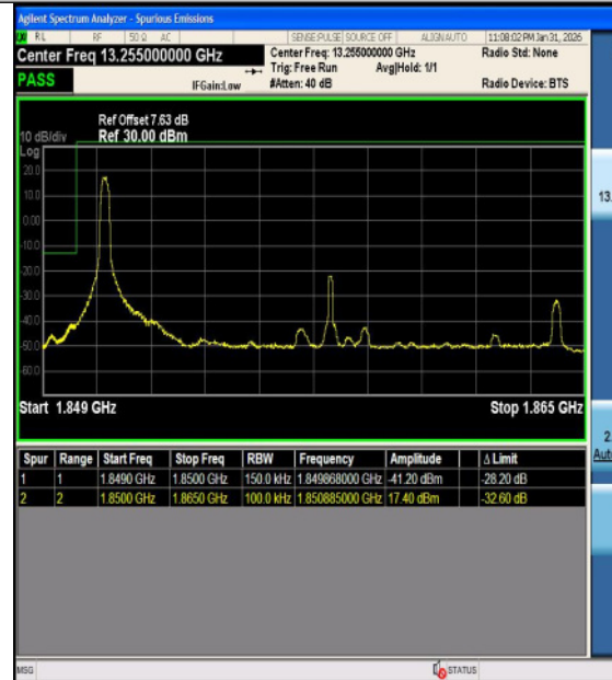
Band2-15MHz-16QAM-18675-75RB#0-PASS
