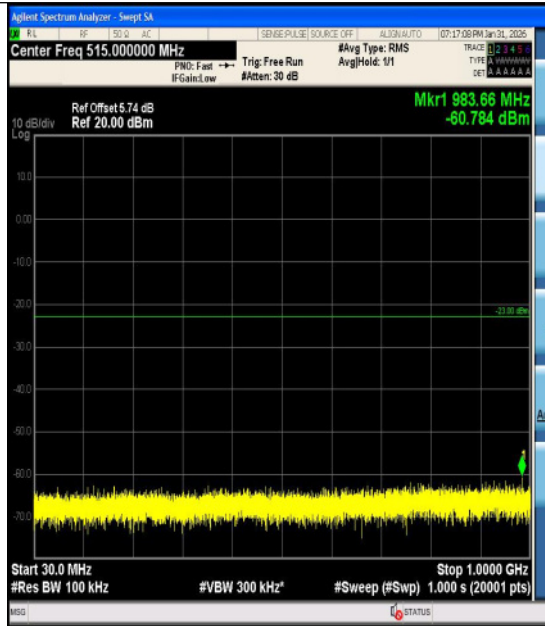
Band2-3MHz-16QAM-18615-1RB#0-3000~2000 0-PASS
