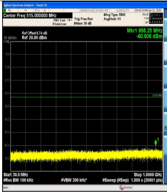
Band2-5MHz-16QAM-18625-25RB#0-3000~200 00-PASS
