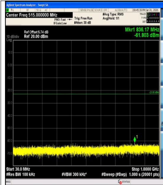
Band2-5MHz-QPSK-18900-25RB#0-3000~2000 0-PASS
