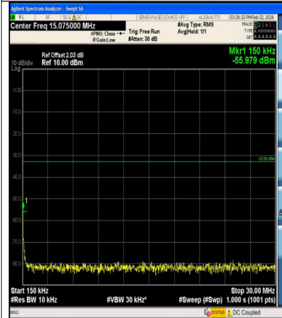
Band4-5MHz-16QAM-20375-1RB#0-1000~3000-
