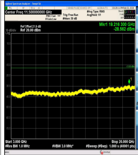
Band4-5MHz-16QAM-20375-25RB#0-0.15~30-P ASS
