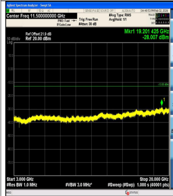
Band4-15MHz-QPSK-20025-1RB#74-0.15~30-P ASS
