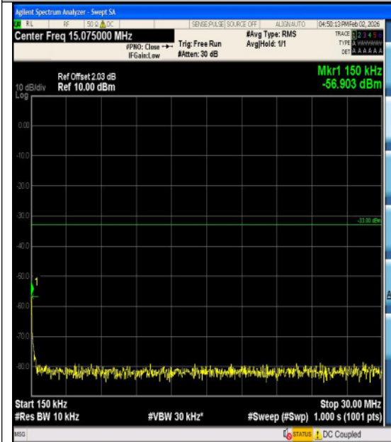
Band4-15MHz-16QAM-20025-1RB#0-1000~300 0-PASS
