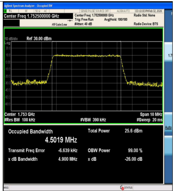
Band4-10MHz-16QAM-20000-50RB#0-PASS
