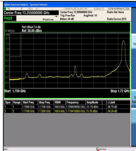
Band4-10MHz-16QAM-20000-1RB#0-PASS
