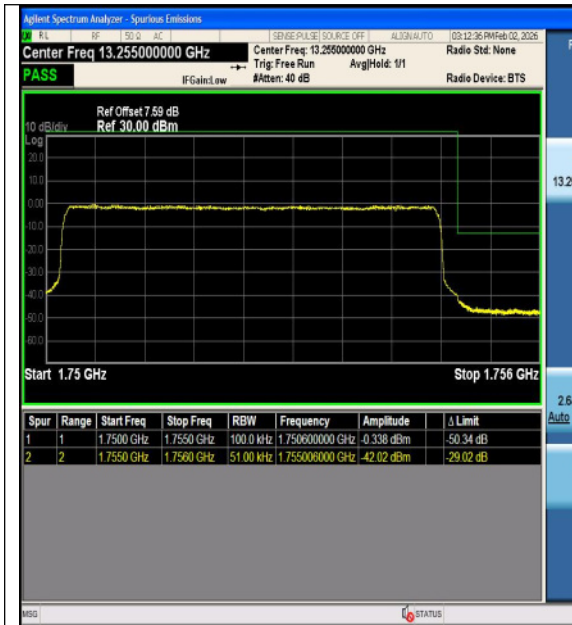
Band4-5MHz-16QAM-20375-1RB#24-PASS
