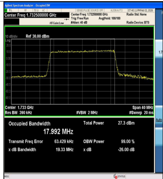
Band4-20MHz-16QAM-20300-100RB#0-PASS
