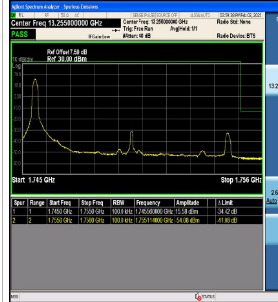
Band4-10MHz-QPSK-20350-50RB#0-PASS
