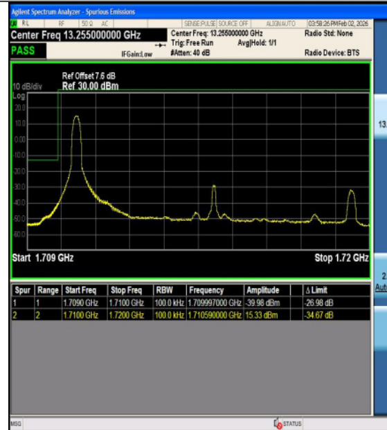
Band4-10MHz-16QAM-20000-50RB#0-PASS
