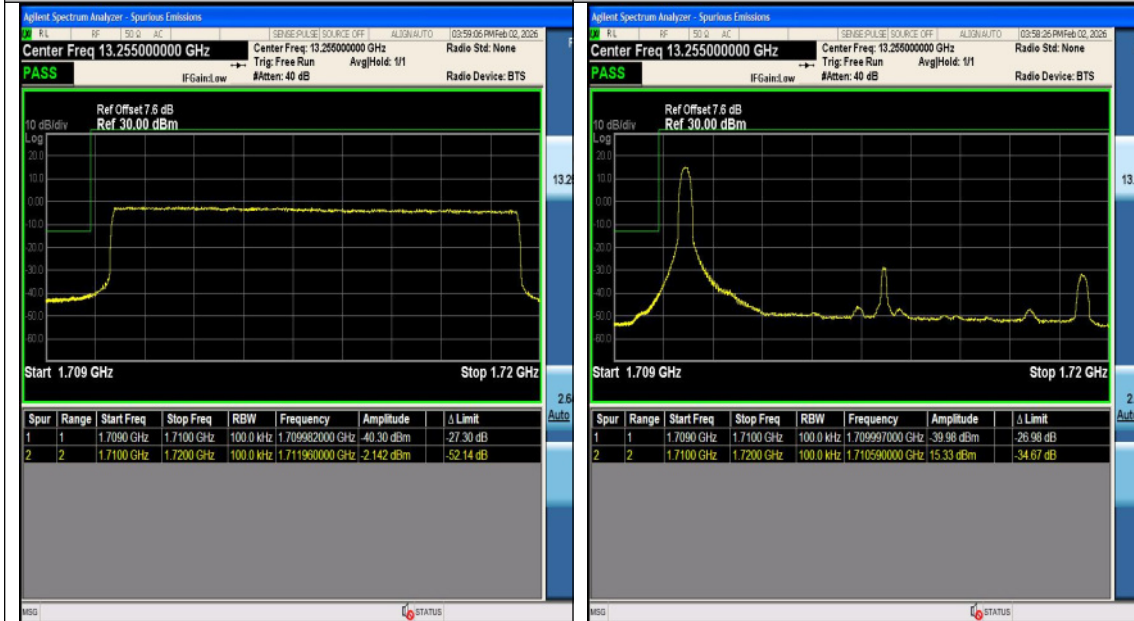
Band4-10MHz-16QAM-20000-1RB#49-PASS
