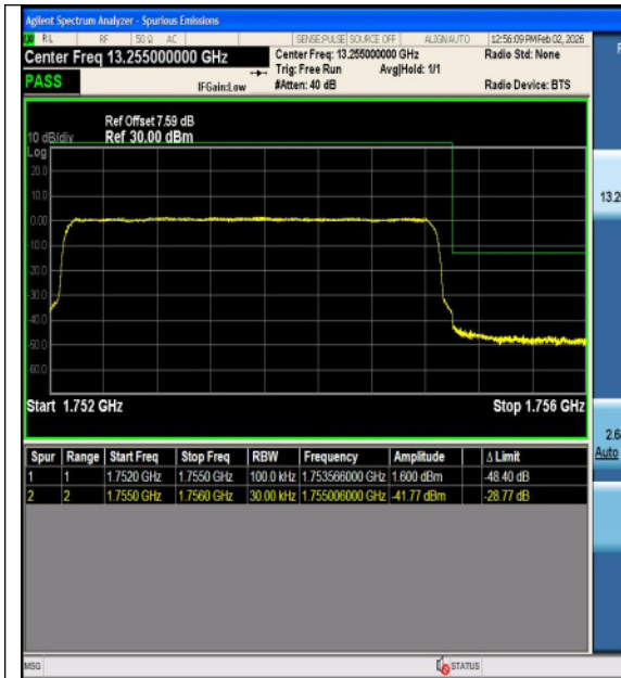
Band4-3MHz-16QAM-20385-1RB#14-PASS
