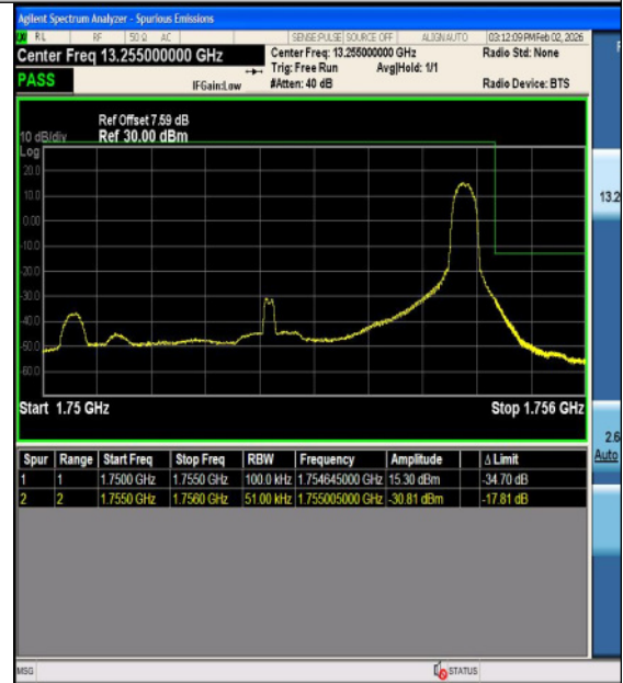
Band4-5MHz-16QAM-20375-1RB#0-PASS
