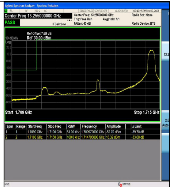
Band4-5MHz-16QAM-19975-1RB#0-PASS
