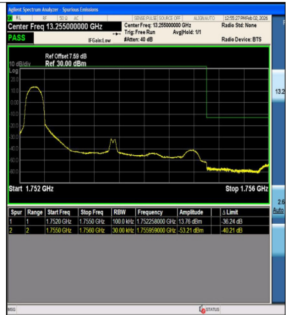
Band4-3MHz-16QAM-20385-15RB#0-PASS
