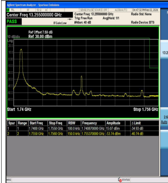
Band4-15MHz-QPSK-20325-75RB#0-PASS
