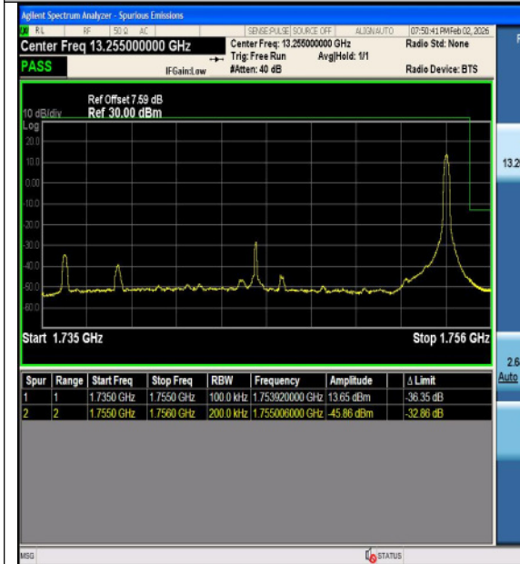
Band4-20MHz-16QAM-20300-1RB#99-PASS
