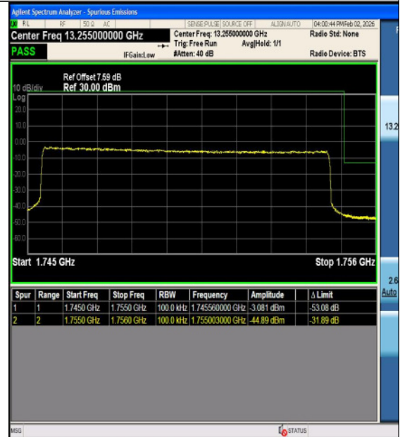
Band4-15MHz-QPSK-20025-1RB#74-PASS
