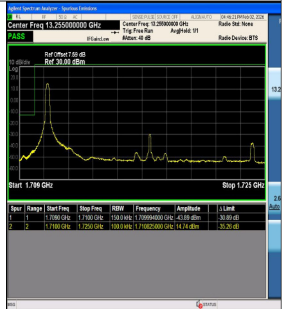
Band4-15MHz-16QAM-20025-75RB#0-PASS
