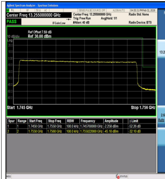
Band4-10MHz-16QAM-20350-1RB#49-PASS
