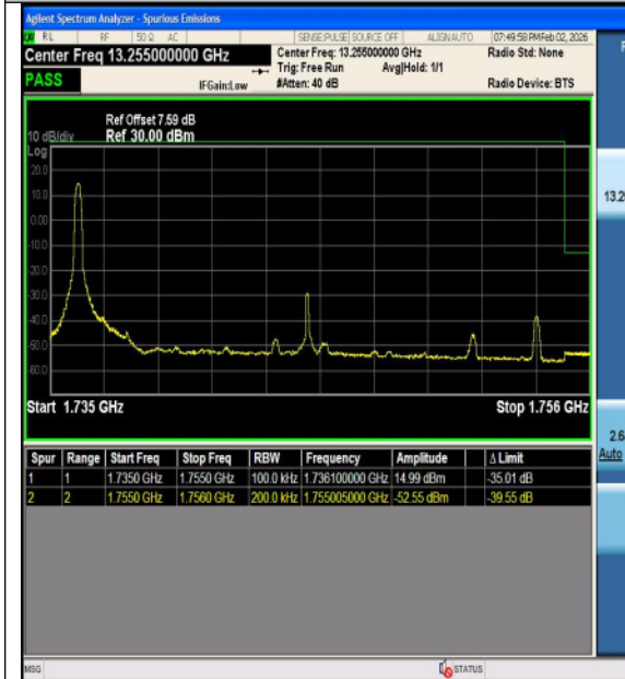
Band4-20MHz-QPSK-20300-100RB#0-PASS
