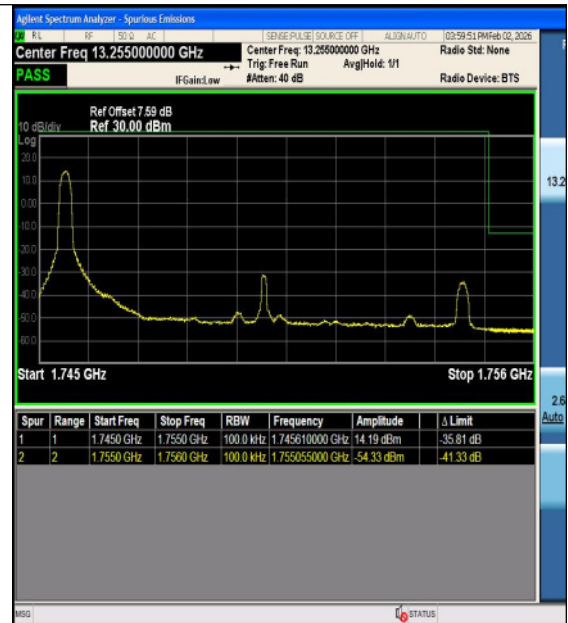
Band4-10MHz-16QAM-20350-50RB#0-PASS
