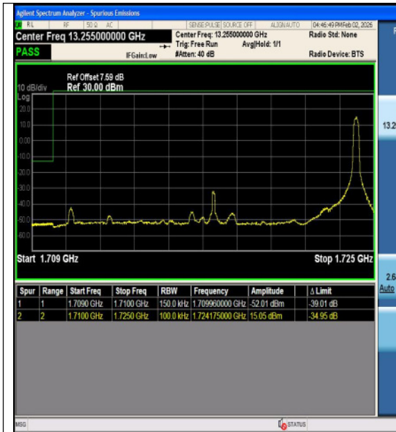
Band4-15MHz-QPSK-20325-1RB#0-PASS
