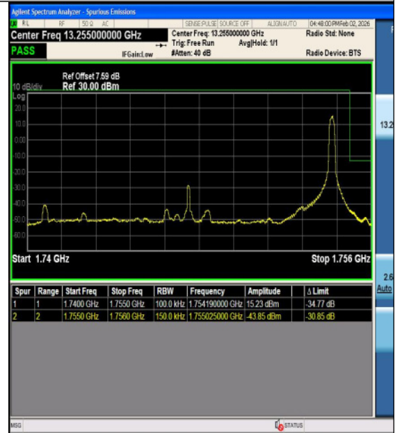
Band4-15MHz-16QAM-20325-1RB#0-PASS
