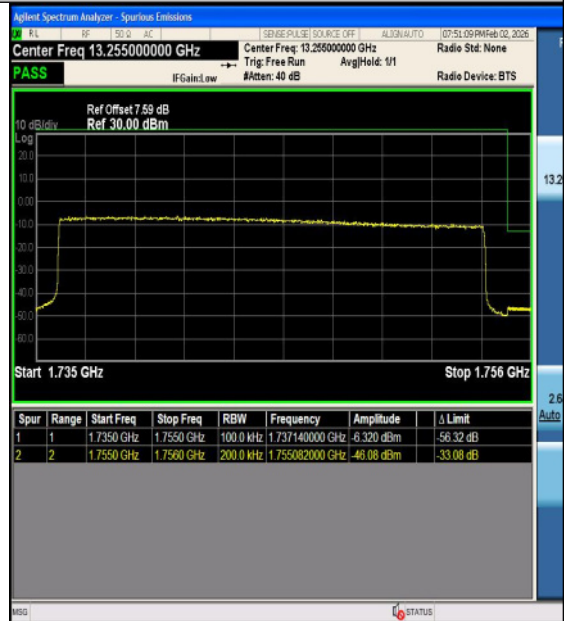
Band4-20MHz-16QAM-20300-100RB#0-PASS
