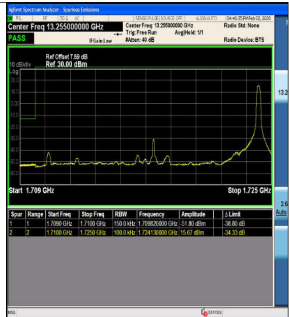
Band4-15MHz-16QAM-20025-1RB#0-PASS
