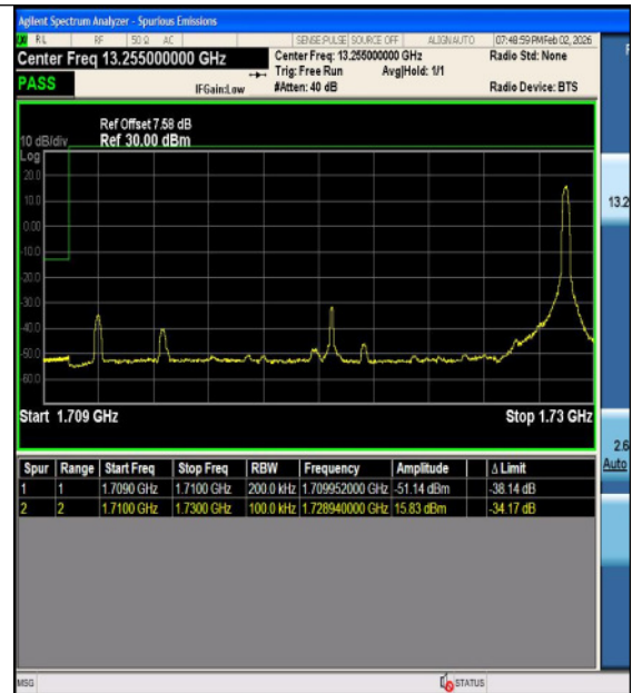
Band4-20MHz-16QAM-20050-1RB#0-PASS
