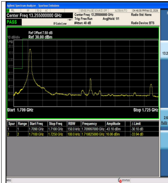
Band4-15MHz-QPSK-20025-75RB#0-PASS
