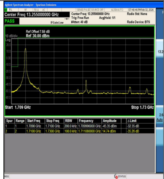
Band4-20MHz-16QAM-20050-100RB#0-PASS
