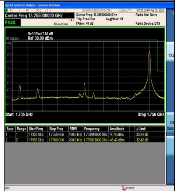
Band4-20MHz-16QAM-20300-1RB#0-PASS
