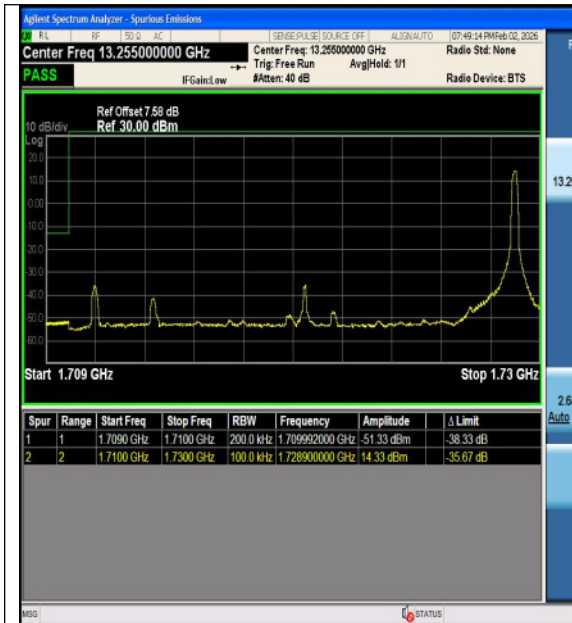
Band4-20MHz-QPSK-20300-1RB#0-PASS
