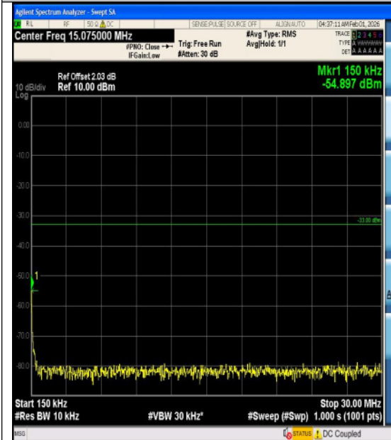
Band4-1.4MHz-16QAM-20175-6RB#0-1000~3000 0-PASS
