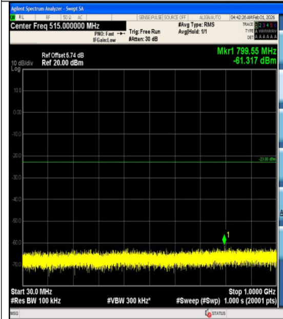
Band4-1.4MHz-QPSK-20393-6RB#0-3000~2000 0-PASS
