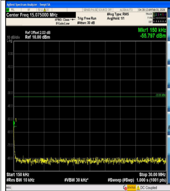
Band4-1.4MHz-16QAM-20393-1RB#0-1000~3000 0-PASS
