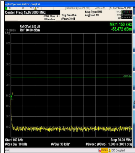
Band4-3MHz-16QAM-20175-1RB#0-1000~3000-
