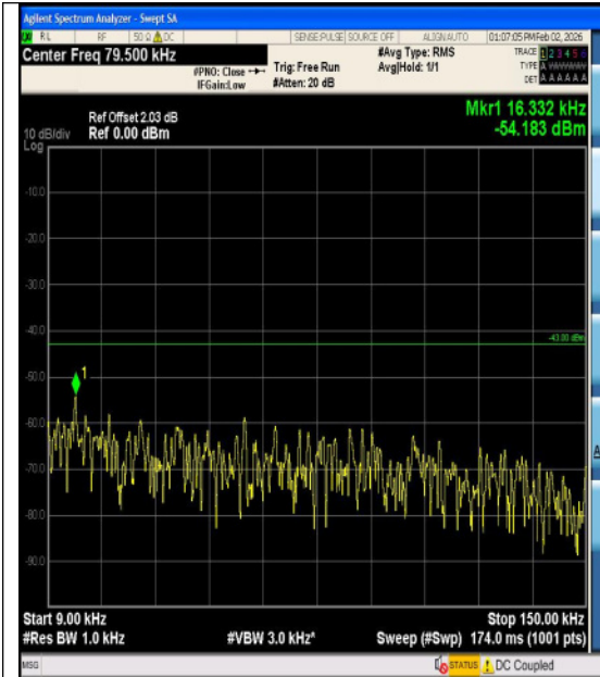
Band4-3MHz-16QAM-19965-1RB#14-30~1000-P ASS
