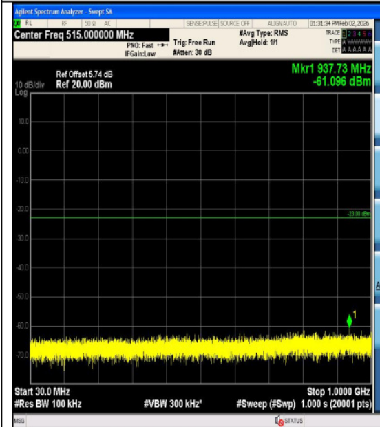
Band4-3MHz-QPSK-20175-15RB#0-3000~2000 0-PASS
