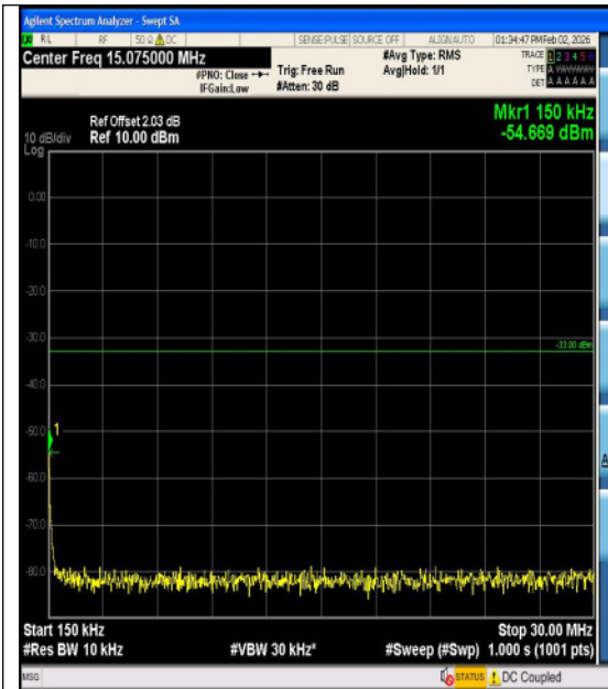
Band4-3MHz-16QAM-20175-15RB#0-1000~300 0-PASS
