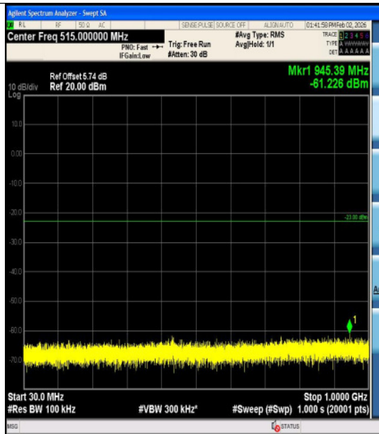
Band4-3MHz-16QAM-20385-1RB#0-3000~2000 0-PASS
