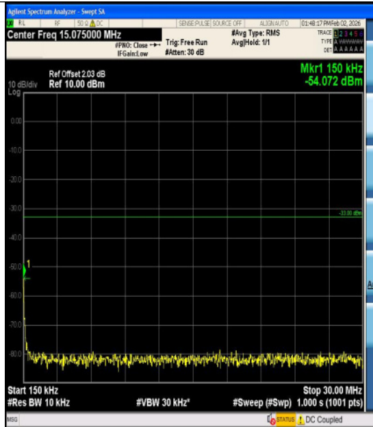
Band4-3MHz-16QAM-20385-1RB#14-1000~300 0-PASS
