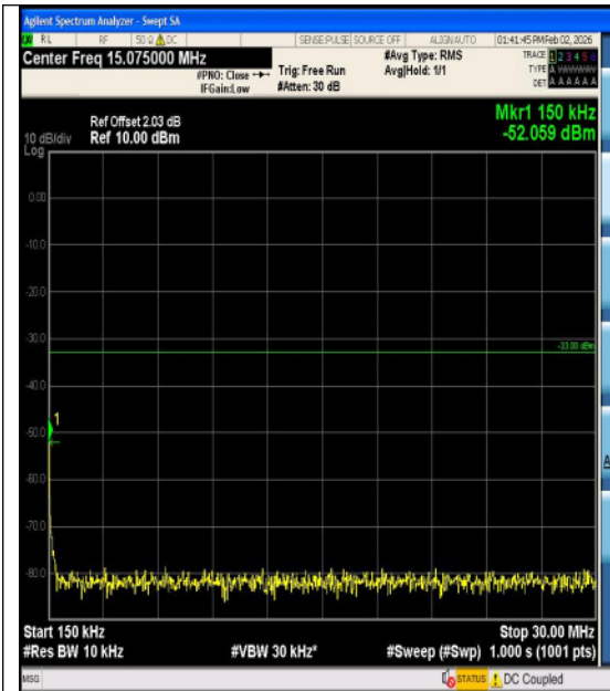
Band4-3MHz-16QAM-20385-1RB#0-1000~3000- PASS
