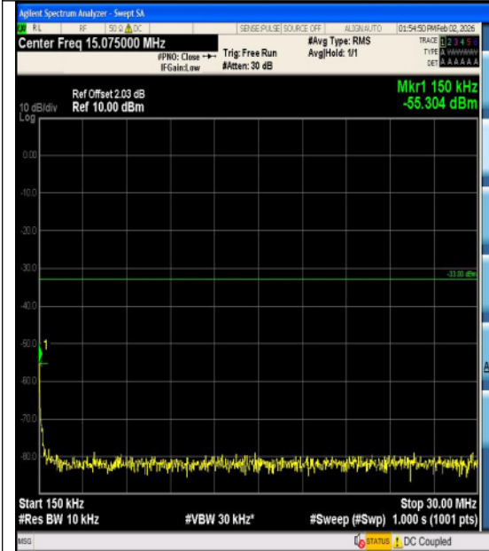
Band4-3MHz-16QAM-20385-15RB#0-1000~300 0-PASS
