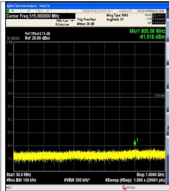
Band4-5MHz-QPSK-20175-25RB#0-3000~2000 0-PASS
