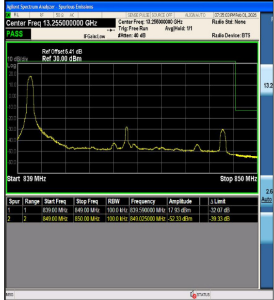
Band5-10MHz-16QAM-20600-50RB#0-PASS
