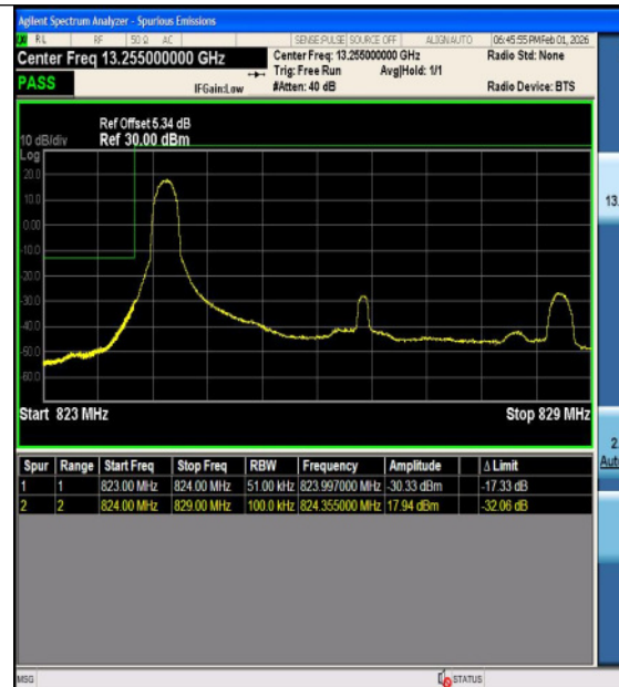
Band5-5MHz-16QAM-20425-25RB#0-PASS
