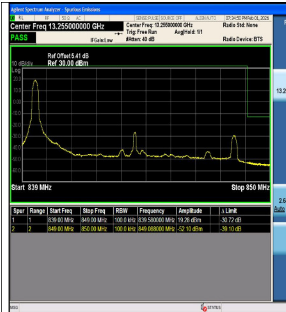
Band5-10MHz-QPSK-20600-50RB#0-PASS
