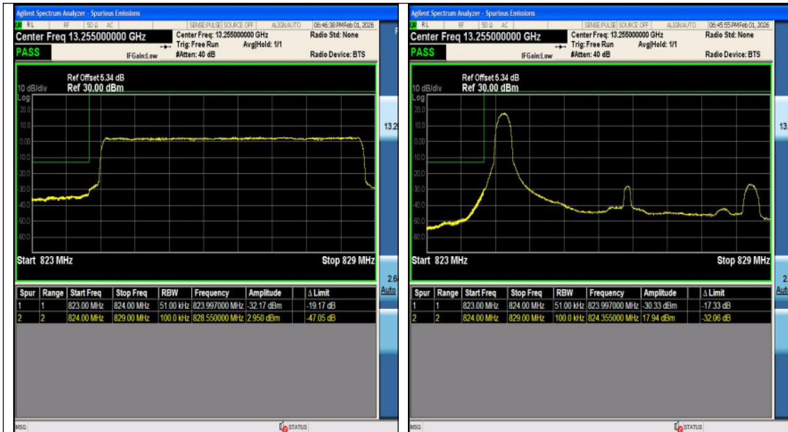
Band5-5MHz-16QAM-20425-1RB#24-PASS
