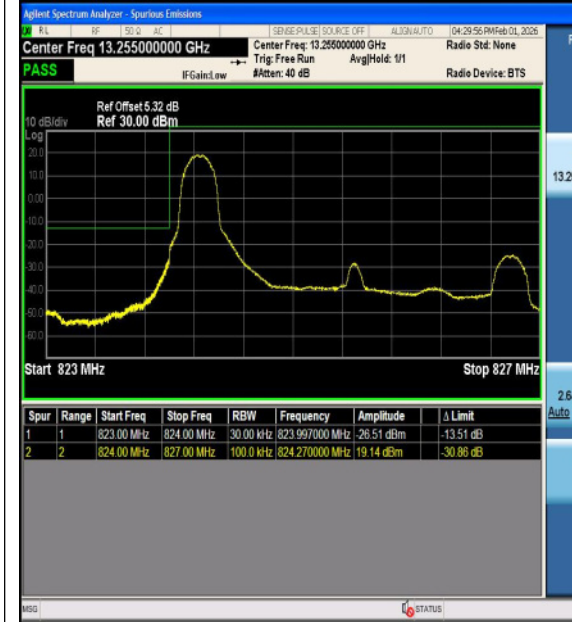
Band5-3MHz-QPSK-20415-15RB#0-PASS
