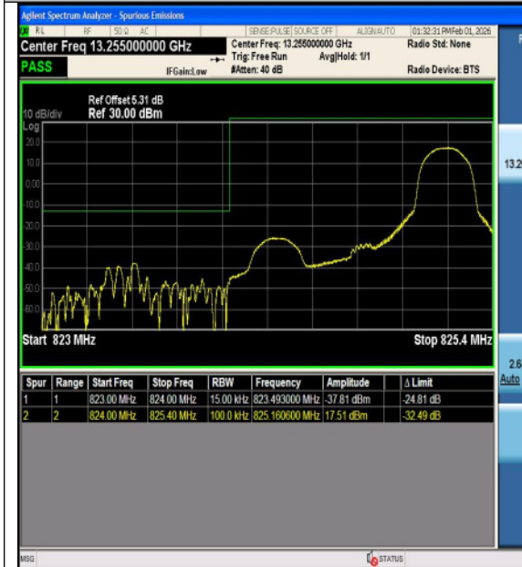
Band5-1.4MHz-QPSK-20643-1RB#0-PASS
