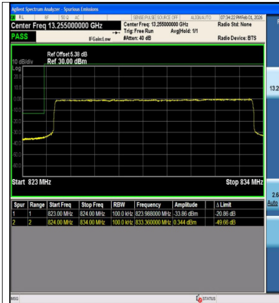
Band5-10MHz-16QAM-20450-1RB#49-PASS
