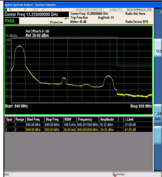
Band5-3MHz-16QAM-20635-15RB#0-PASS
