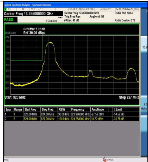
Band5-3MHz-16QAM-20415-15RB#0-PASS
