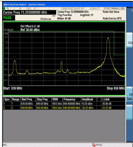
Band5-10MHz-16QAM-20600-1RB#0-PASS
