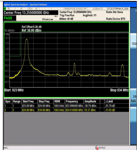
Band5-10MHz-16QAM-20450-50RB#0-PASS
