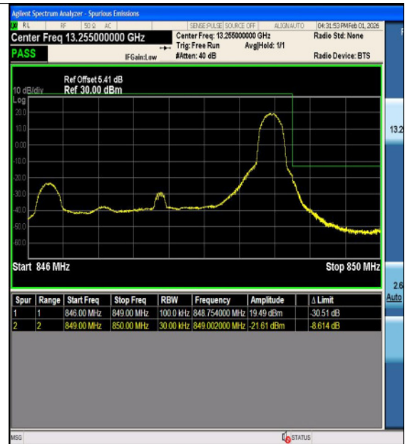
Band5-3MHz-16QAM-20635-1RB#0-PASS
