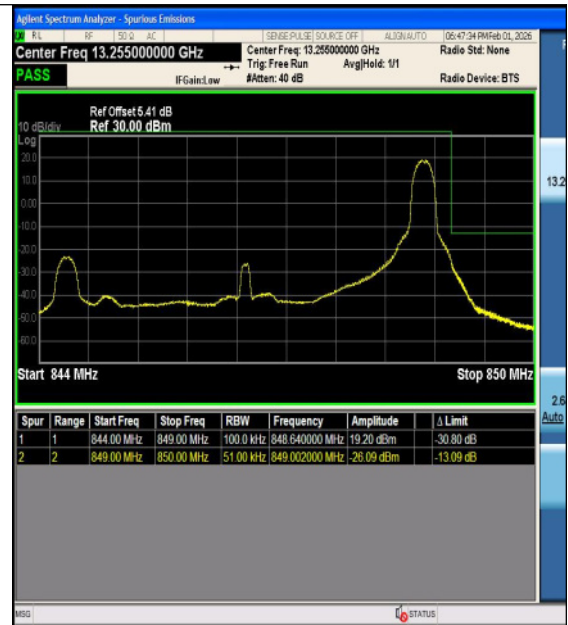
Band5-5MHz-16QAM-20625-1RB#0-PASS
