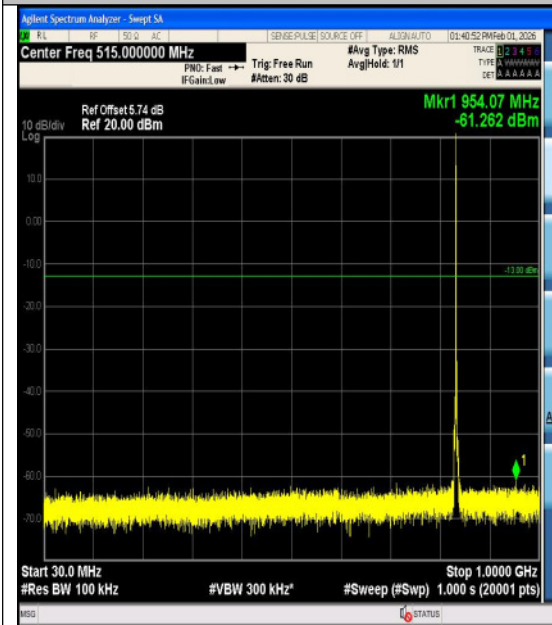
Band5-1.4MHz-QPSK-20525-1RB#0-3000~1000 0-PASS
