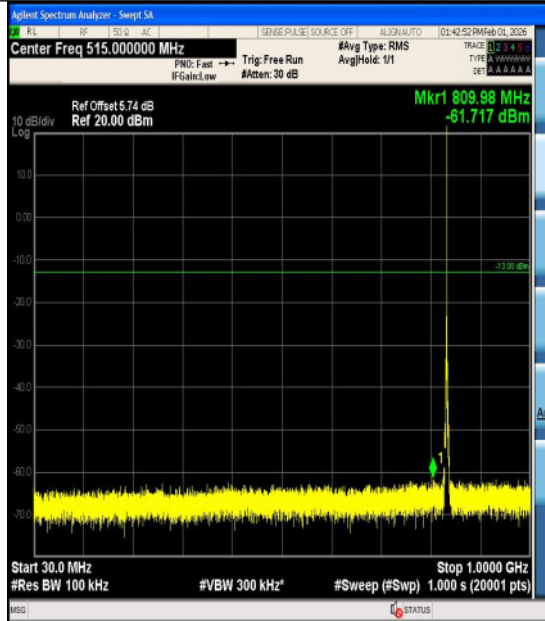
Band5-1.4MHz-QPSK-20525-1RB#5-3000~1000 0-PASS
