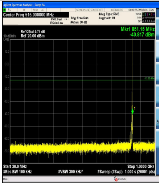
Band5-1.4MHz-QPSK-20643-1RB#5-3000~1000 0-PASS
