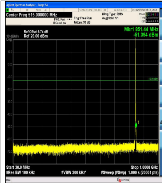
Band5-1.4MHz-QPSK-20643-1RB#0-3000~1000 0-PASS
