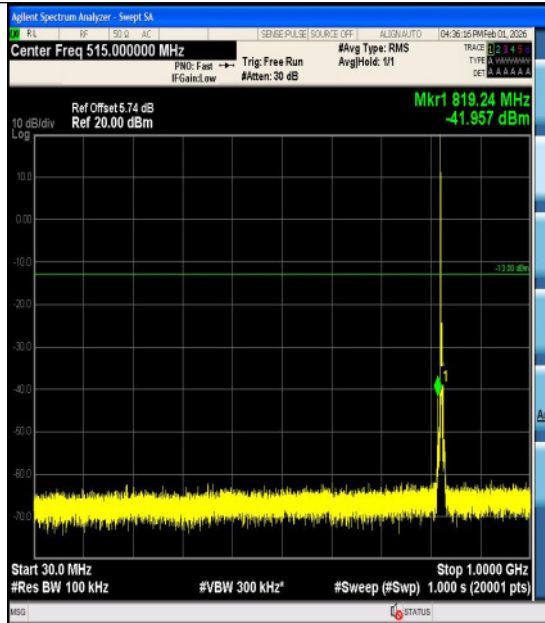
Band5-3MHz-16QAM-20415-1RB#0-3000~1000 0-PASS
