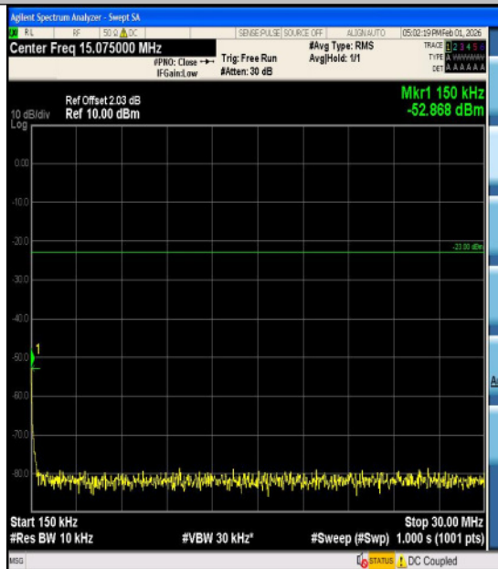
Band5-3MHz-16QAM-20525-1RB#14-1000~300 0-PASS
