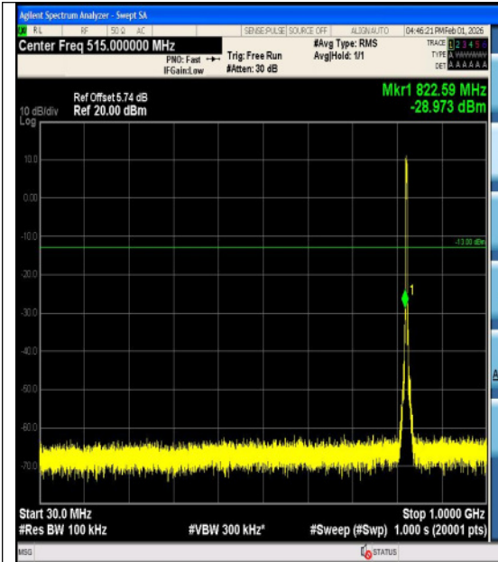
Band5-3MHz-QPSK-20415-15RB#0-3000~1000 0-PASS
