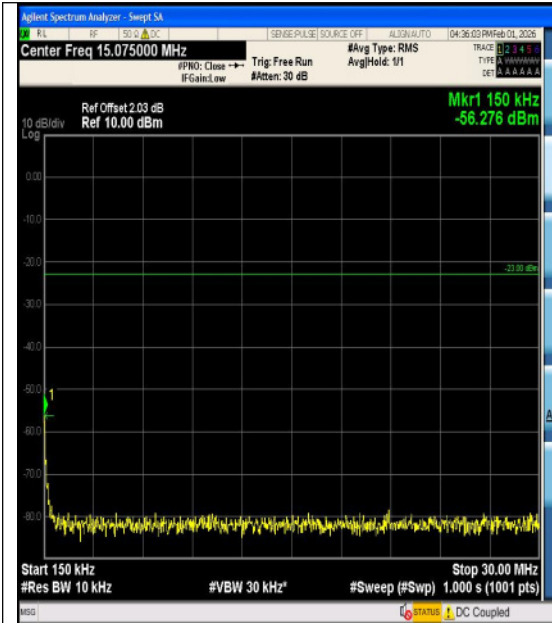
Band5-3MHz-16QAM-20415-1RB#0-1000~3000- PASS
