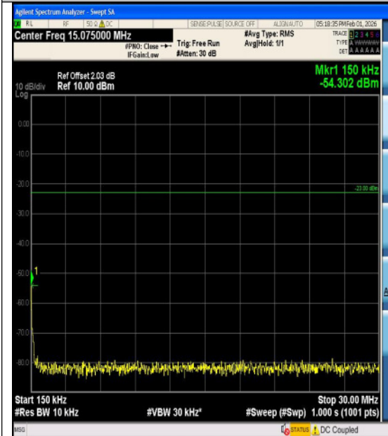
Band5-3MHz-QPSK-20635-1RB#14-1000~3000- PASS
