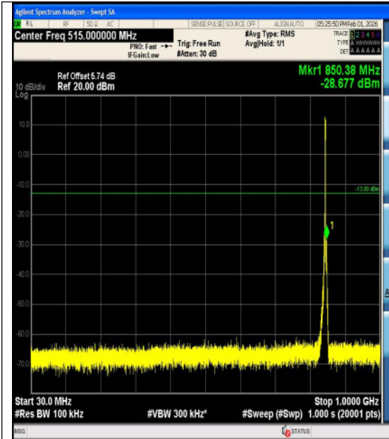
Band5-3MHz-QPSK-20635-15RB#0-3000~1000 0-PASS
