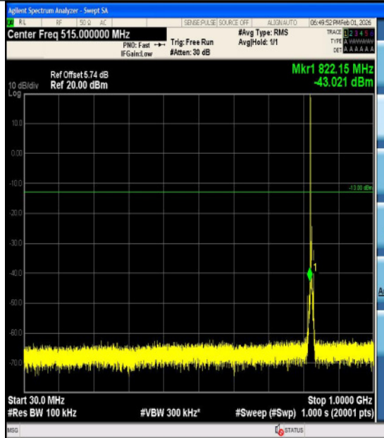
Band5-5MHz-16QAM-20425-1RB#0-3000~1000 0-PASS
