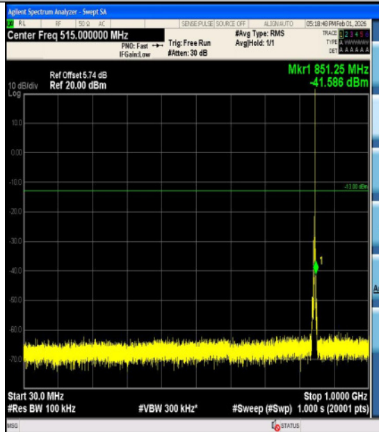
Band5-3MHz-QPSK-20635-1RB#14-3000~1000 0-PASS
