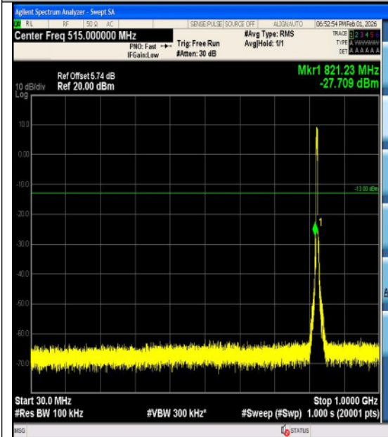
Band5-5MHz-QPSK-20425-25RB#0-3000~1000 0-PASS
