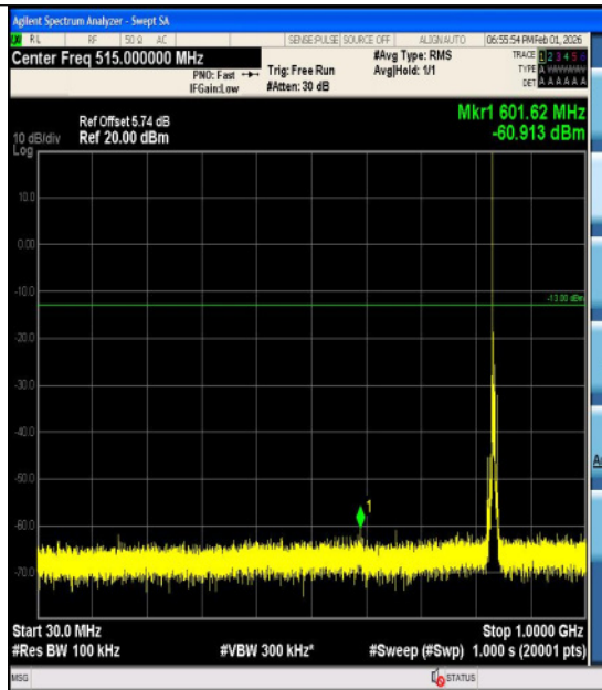
Band5-5MHz-16QAM-20525-1RB#0-3000~1000 0-PASS
