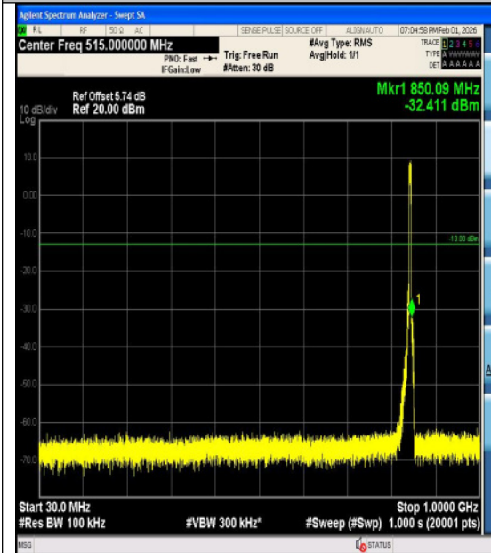
Band5-5MHz-QPSK-20625-25RB#0-3000~1000 0-PASS
