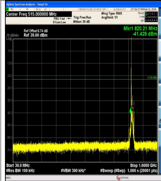
Band5-10MHz-QPSK-20450-1RB#0-3000~1000 0-PASS
