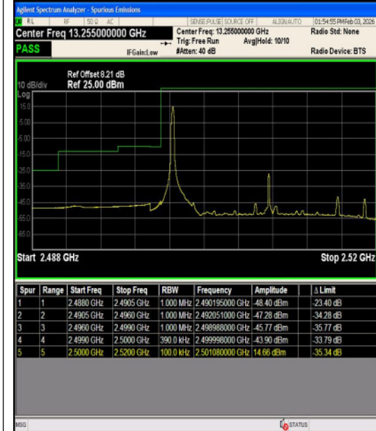
Band7-20MHz-QPSK-20850-100RB#0-PASS
