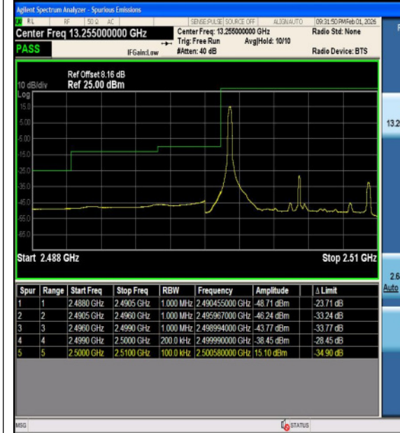
Band7-10MHz-QPSK-20800-50RB#0-PASS
