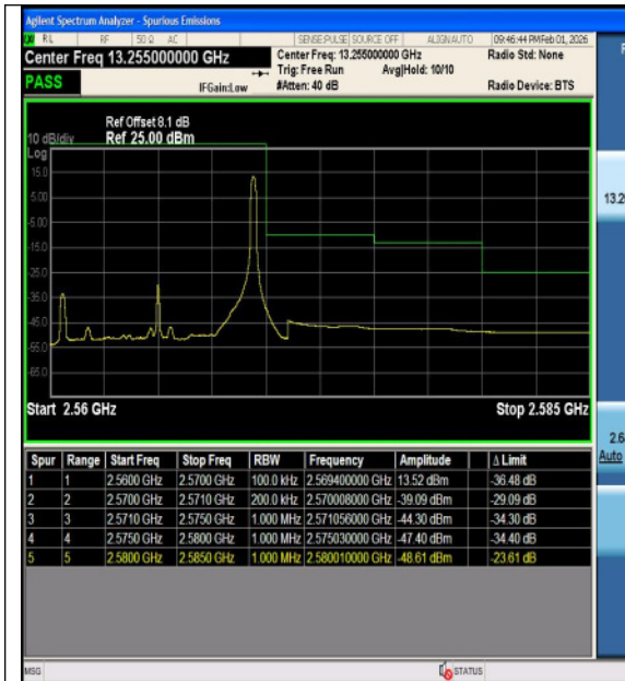
Band7-15MHz-QPSK-20825-1RB#0-PASS
