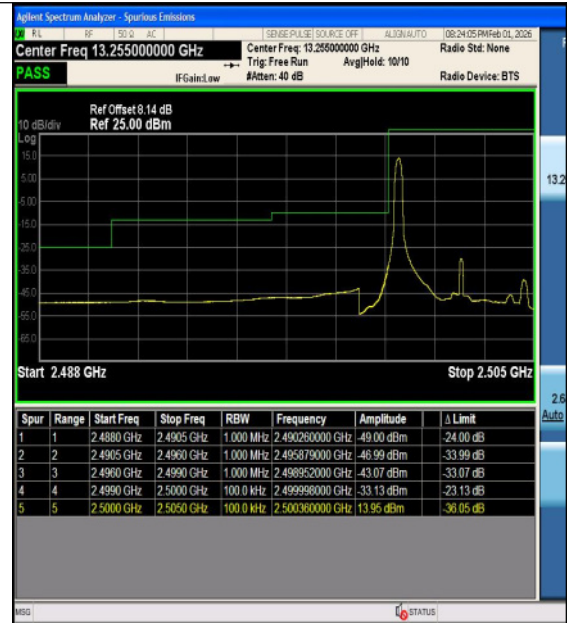
Band7-5MHz-16QAM-20775-25RB#0-PASS
