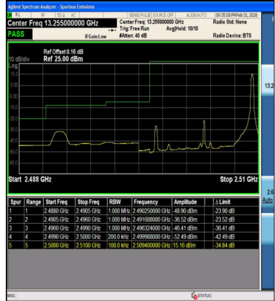
Band7-10MHz-16QAM-20800-1RB#0-PASS
