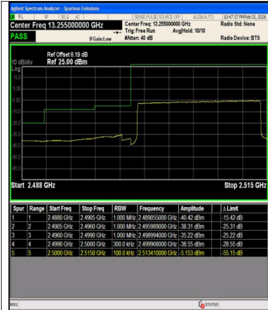
Band7-15MHz-16QAM-20825-1RB#74-PASS
