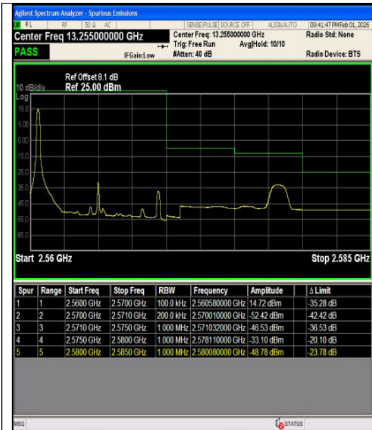
Band7-10MHz-QPSK-21400-50RB#0-PASS
