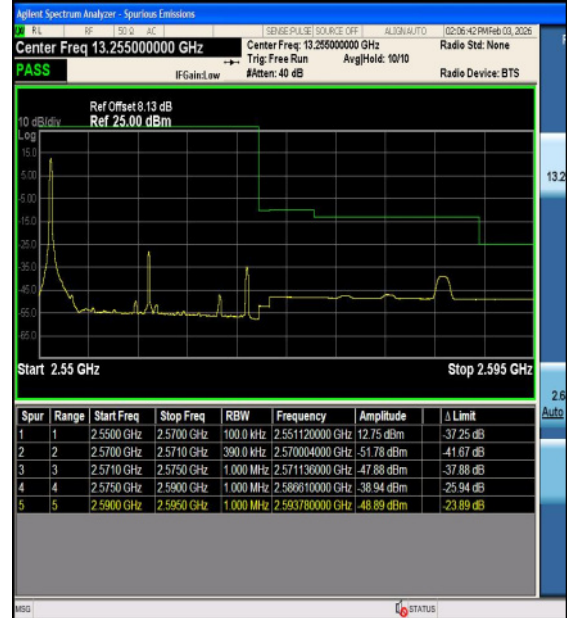
Band7-20MHz-16QAM-21350-100RB#0-PASS
