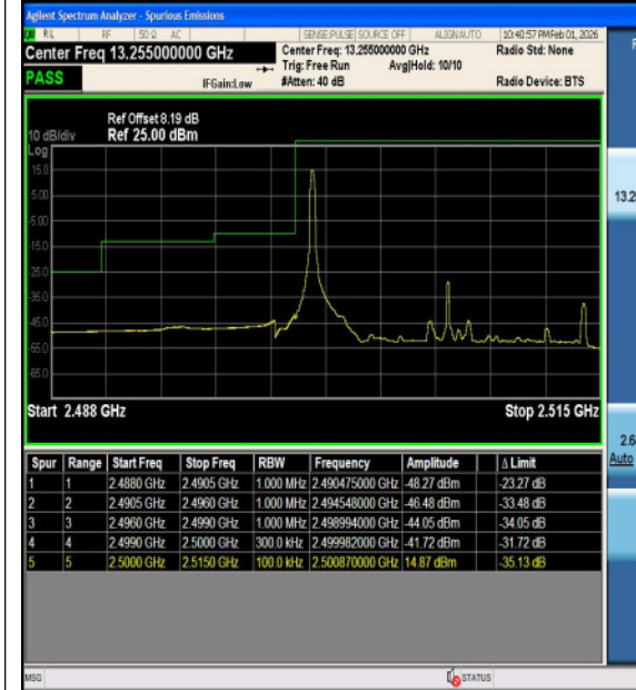
Band7-15MHz-QPSK-20825-75RB#0-PASS
