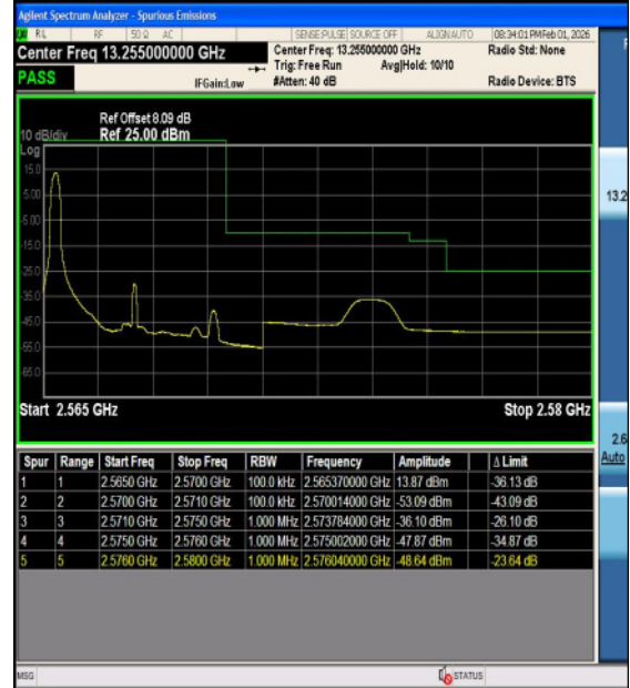
Band7-5MHz-16QAM-21425-25RB#0-PASS
