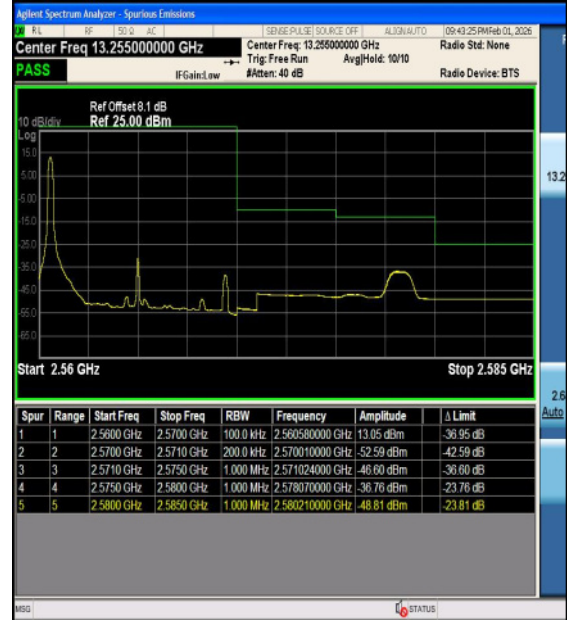
Band7-10MHz-16QAM-21400-50RB#0-PASS
