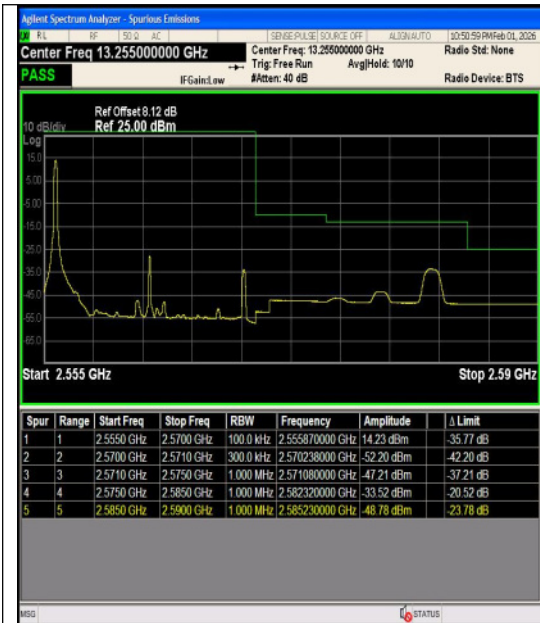
Band7-15MHz-QPSK-21375-75RB#0-PASS
