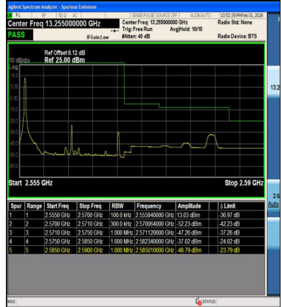
Band7-15MHz-16QAM-21375-75RB#0-PASS
