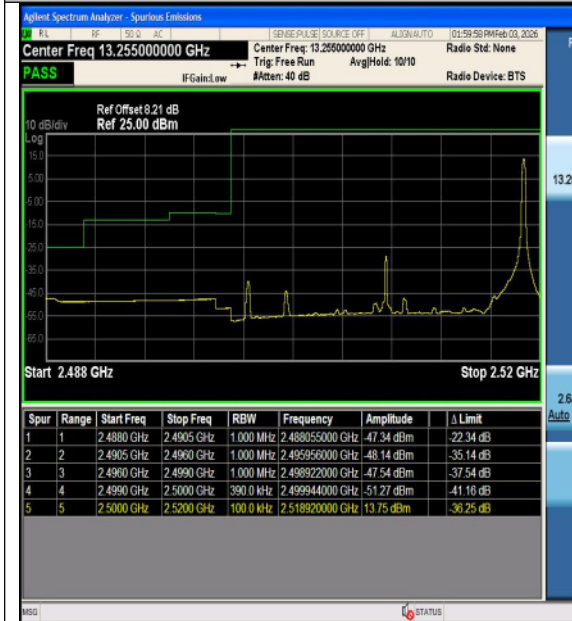
Band7-20MHz-QPSK-21350-1RB#0-PASS
