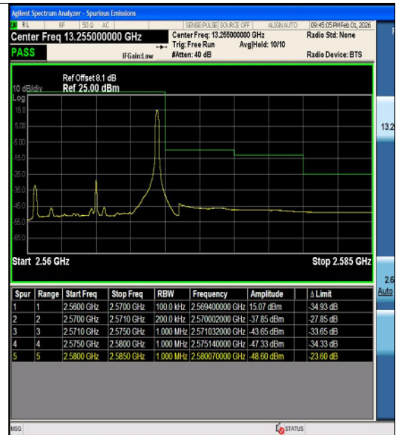
Band7-10MHz-16QAM-21400-1RB#0-PASS
