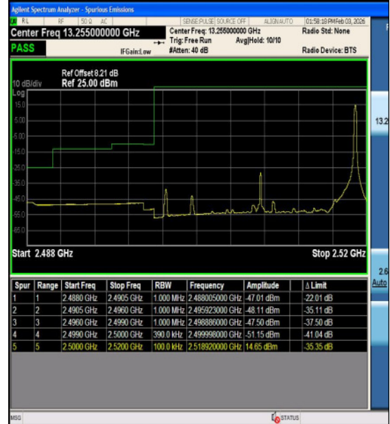
Band7-20MHz-16QAM-20850-1RB#0-PASS
