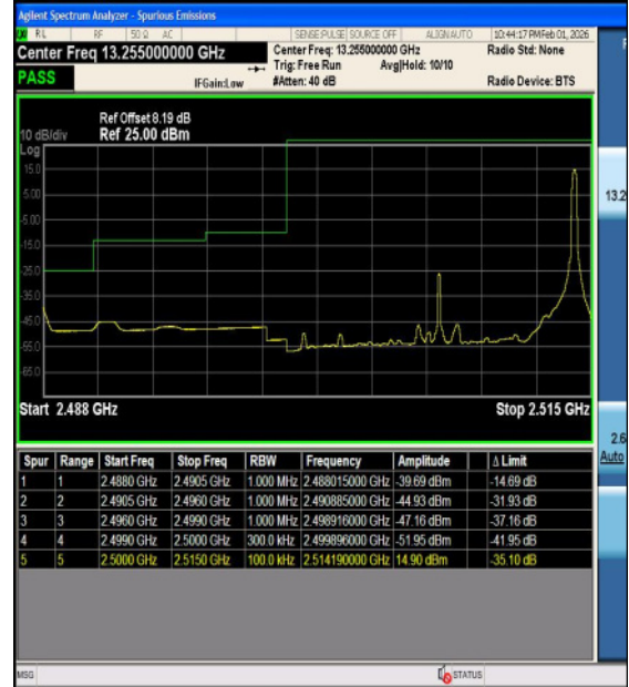
Band7-15MHz-16QAM-20825-1RB#0-PASS
