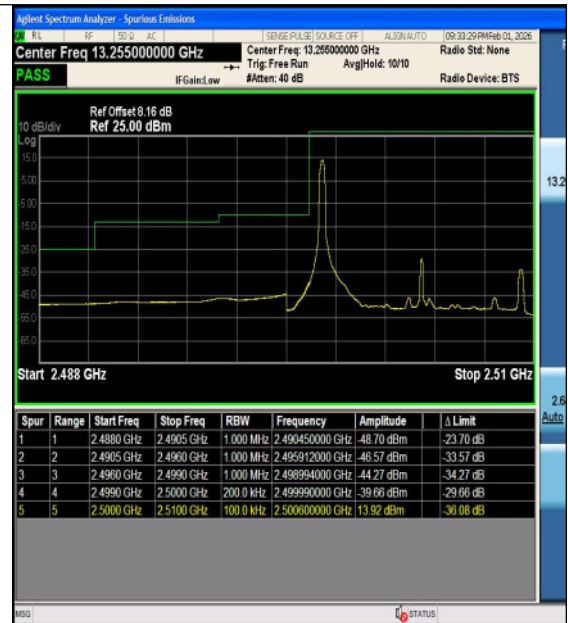
Band7-10MHz-16QAM-20800-50RB#0-PASS
