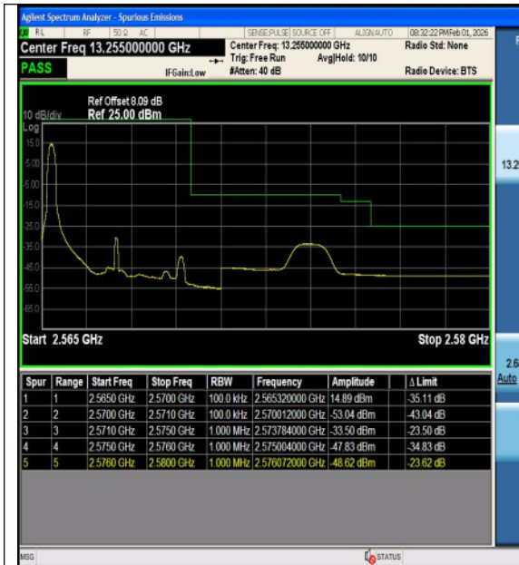
Band7-5MHz-QPSK-21425-25RB#0-PASS
