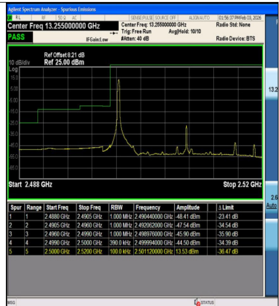
Band7-20MHz-16QAM-20850-100RB#0-PASS
