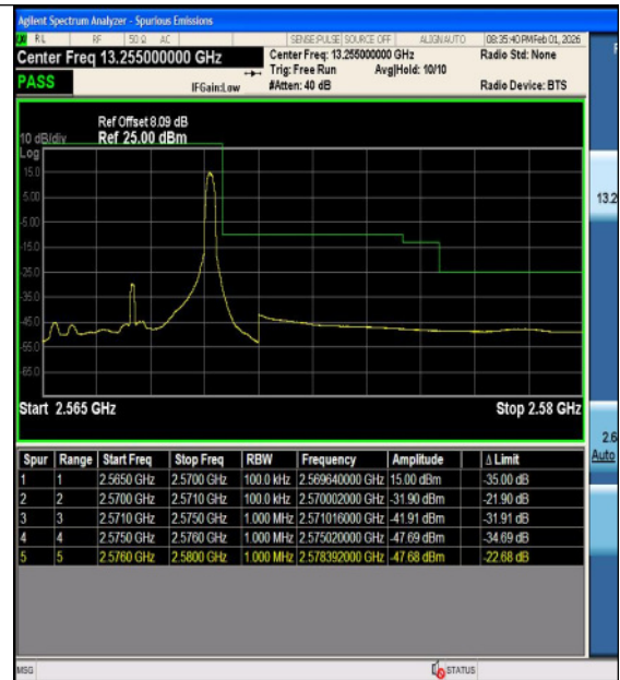
Band7-5MHz-16QAM-21425-1RB#0-PASS
