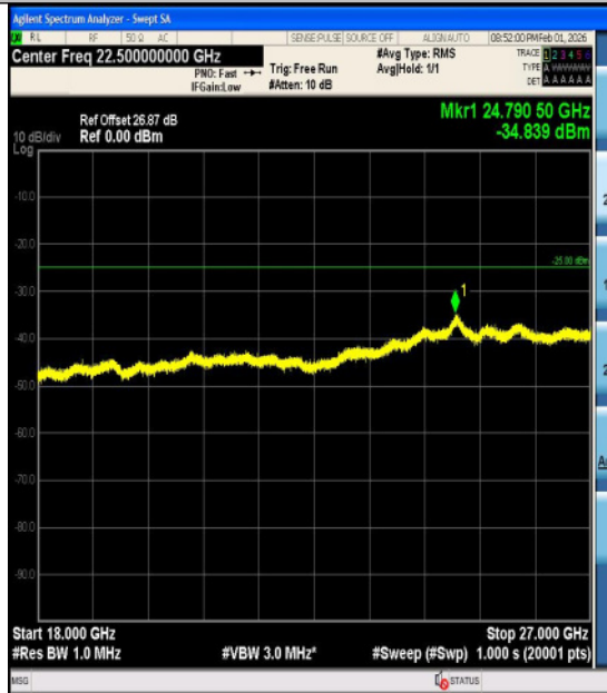
Band7-5MHz-QPSK-21100-25RB#0-0.15~30-PA SS
